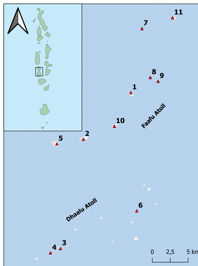
FIGURE 1 The studied 11 islands of the Faafu (north) and Dhaalu (south) atolls. Island full names and coordinates are provided in Table S1. The gradient of green area fragmentation is reported in Figure S1
