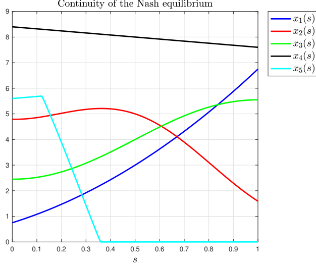
FIGURE 1. Continuity of the Nash equilibrium with respect to parameter s .
