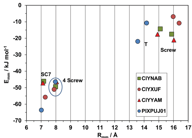
Fig. 7 Energetic profiles (kJ mol -1 ) for a series of strictly isostructural crystals (see Table 1). SC7 = slipped-cofacial with 7 Å translation; 4 screw, coordination by 4 screw related molecules. The upper right part is manifold of closely related symmetries.
