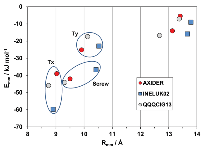
Fig. 8 Energetic profiles (kJ mol -1 ) for a series of almost isostructural crystals (see Table 1). Tx, Ty: translation along cell edges.
