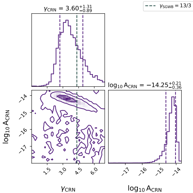
Figure 6. The two-dimensional marginal posterior distribution for the log-amplitude ( \log_{10} A_{\text{CRN}} ) and spectral index ( \gamma_{\text{CRN}} ) of the common uncorrelated signal identified in the MPTA data. The contours represent 1\sigma , 2\sigma and 3\sigma confidence regions of the posteriors, and the values reported above each one-dimensional posterior are the median and corresponding 1\sigma values of the signal parameters. The spectral index of the process is consistent with a value representative of an SGWB, which we have overlaid for ease of comparison (green dashed line).
