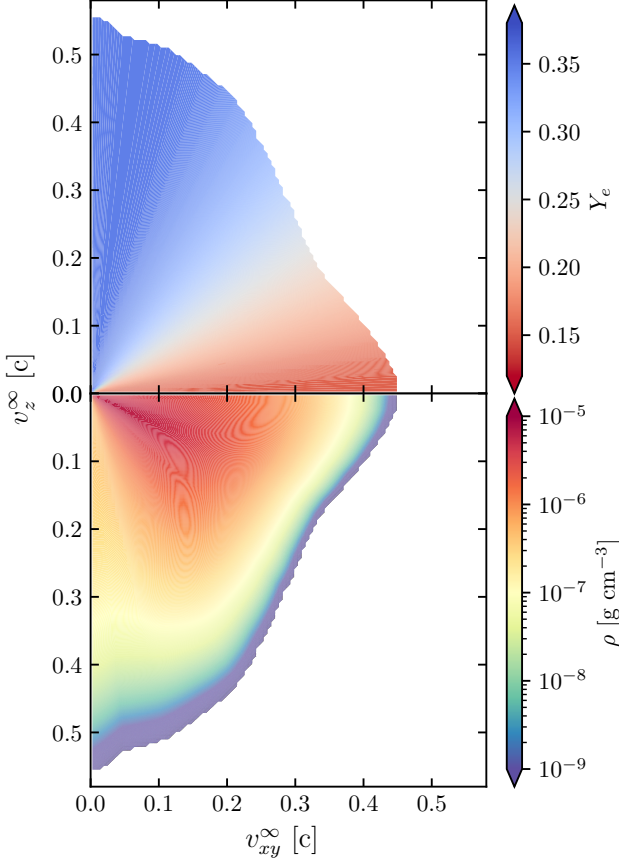
Figure 5. Density and electron fraction distributions in the velocity space for the dynamical ejecta at t = 100 s post-merger. The density radial profile follows the analytic prescription of Eq. (25), while a radially constant electron fraction is assumed. Angular distributions are extracted from the GRHD simulation of an equal-mass BNS system with masses M_{1,2} = 1.364 M_{\odot} using the DD2 EOS (Perego et al. 2019).
