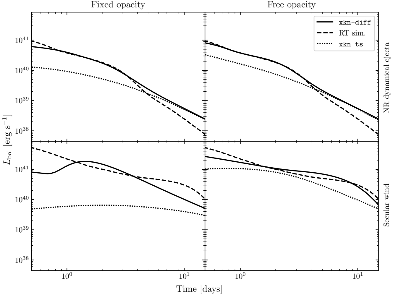
Figure 6. Bolometric luminosity correspondent to the best fit parameters in the dynamical and the secular component configurations, as obtained by using xkn-diff and xkn-ts models, with and without a fixed opacity. Curves are shown in comparison to the data on which the fits are performed, derived from the RT calculations obtained with the code developed in Tanaka & Hotokezaka (2013); Kawaguchi et al. (2018, 2021).
