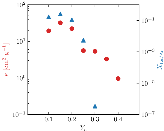
Figure 4. Grey opacity values derived by Tanaka et al. (2020) for temperatures 5000 \text{ K} < T < 10000 \text{ K} and densities \rho \sim 10^{-13} \text{ g cm}^{-3} and for different ejecta compositions characterized by a specific value of electron fraction. The mass fraction of Lanthanides and Actinides is reported for every considered composition.
