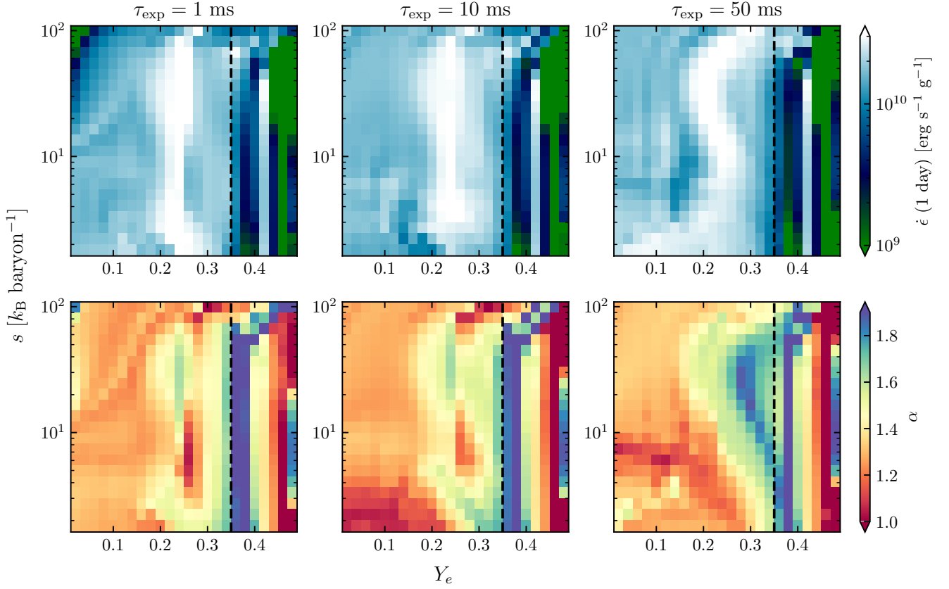
Figure 2. Heating rate fit parameters as functions of the initial electron fraction Y_e and entropy s , for fixed values of the expansion timescale \tau_{\text{exp}} . The dashed line separates the region where we interpolate the parameters linearly (left) from the region where the continuity of the parameters is poor and we use a nearest-point interpolation (right).
