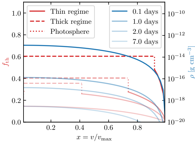
Figure 3. Constructed thermalization efficiency radial profile at different days post-merger. The ejecta density radial profile from Eq. (25) is shown as reference.
