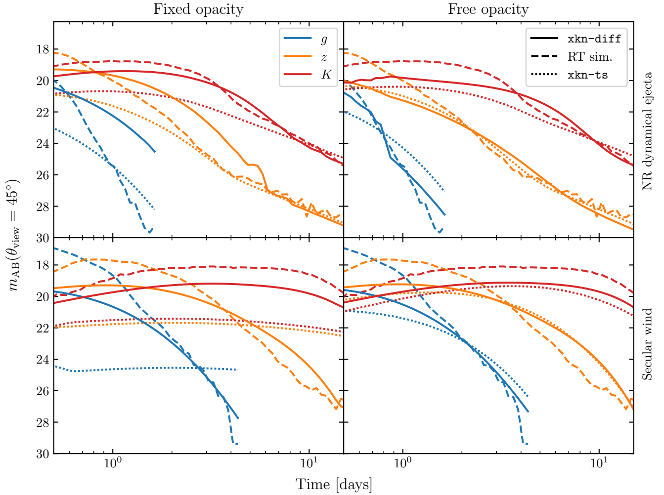
Figure 7. AB magnitudes in the g , z and K filters as seen from a viewing angle \theta_{\text{view}} = 45^\circ , calculated for the best fit parameters in the dynamical and the secular component configurations, using xkn-diff and xkn-ts models, with and without a fixed opacity. Curves are shown in comparison to the data on which the fits were performed, derived from the RT calculations obtained with the code developed in Tanaka & Hotokezaka (2013); Kawaguchi et al. (2018, 2021).
