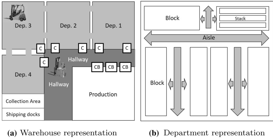
Fig. 1 Warehouse and department representation
