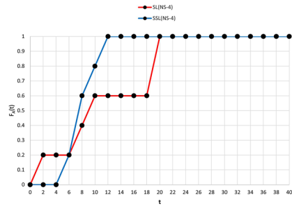
(d) NS-4: performance profiles of the matheuristic with SL and SSL with respect to percentage optimality gap.
