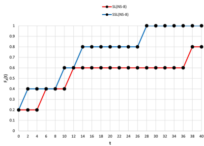
(c) NS-8: performance profiles of the matheuristic with SL and SSL with respect to percentage optimality gap.
