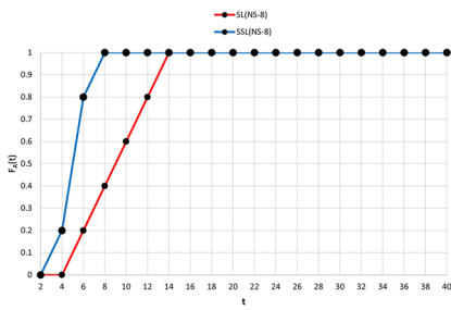
(a) NS-8: performance profiles of the matheuristic with SL and SSL with respect to solving time.
