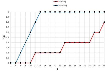
(b) NS-4: performance profiles of the matheuristic with SL and SSL with respect to solving time.
