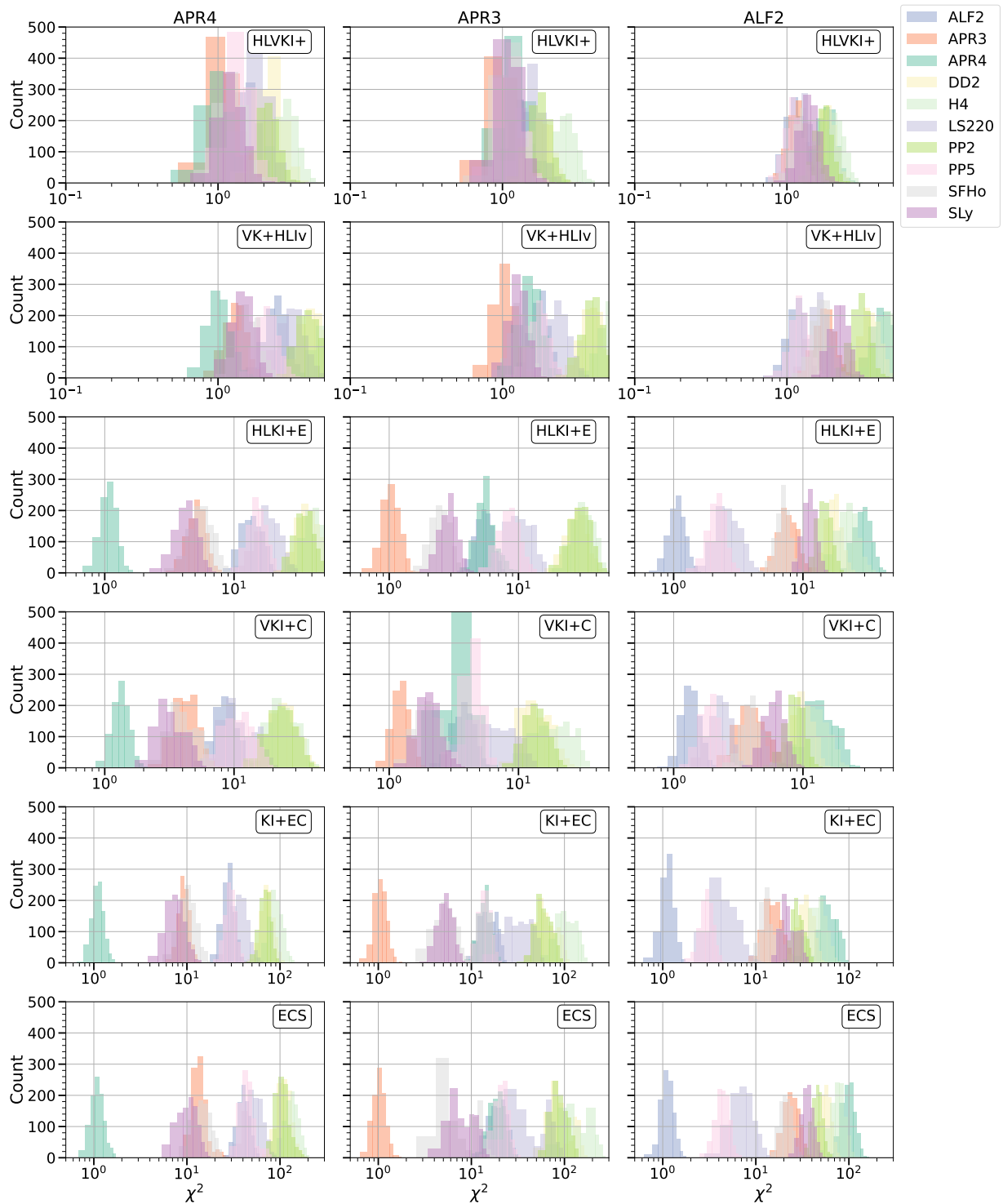
FIG. 6. Chi-square histograms for 100 events from those 500 with the smallest error in combined tidal deformability. The injected EOS is listed along the top, and the colored histograms represent the result assuming a second EOS model, including the original injection. Detector networks are organized by sensitivity row-wise with the most sensitive network at the bottom. In every EOS and network scenario including at least one XG detector, the injected EOS is recovered correctly and easily distinguishable from the other nine via this test. In our two least sensitive and nearest future detector networks, HLVKI+ and VK+HLiv, the opposite is clearly true and all models are indistinguishable.
