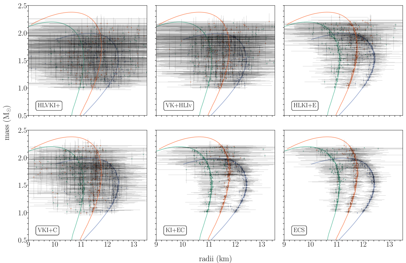
FIG. 4. TOV mass-radius curves of ALF2(blue), APR3(orange), and APR4(green) overlaid with the bias-corrected recovered mass and radius as well as their errors (grey bars) in a subset of near-future and XG detector networks, for a set of 100 random events drawn from the 500 loudest SNR. There is a clear trend of improving radius error as the detector networks improve left to right, top to bottom. Additionally, in the best detector networks, radius errors also improve with decreasing mass, as is to be expected with higher accuracy in the measurement of higher tidal deformability.
