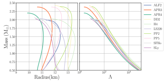
FIG. 1. Mass-Radius curves for EOS used in this paper. Please note that our choice of three injections EOS here (ALF2, APR3, APR4 shown with thicker lines) are motivated by the conservative constraint on \Lambda_{1.4} < 800 as put forward by [79]. We also consider the fact that these three EOS covers a significant range in the maximum masses while the inclusion of additional seven EOS provide good coverage of the rest of the mass radius space.
