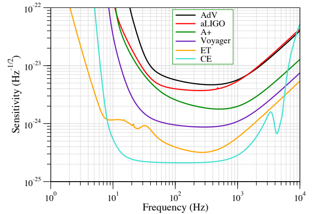
FIG. 2. Strain sensitivity of three generations of ground-based gravitational wave detectors: (i) Advanced Virgo (AdV), Advanced LIGO (aLIGO) and A+, (ii) Voyager, and (iii) Einstein Telescope (ET) and Cosmic Explorer (CE). In the case of ET the sensitivity shown is that of an L-shaped detector with 10 km arms. The three V-shaped arms make the effective strain sensitivity a factor 3/2 better (and the noise floor lower by the same factor).
