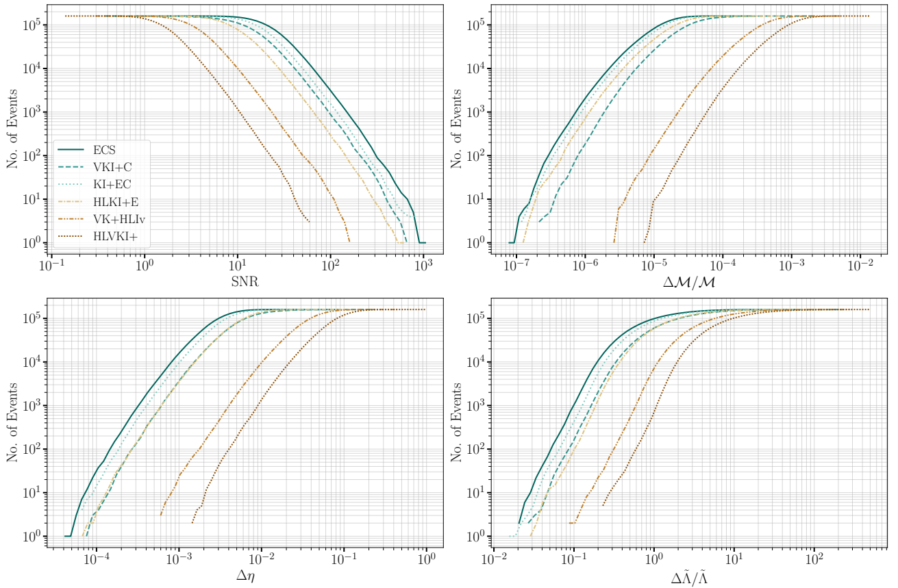
FIG. 3. This plot shows the distribution of the measurement accuracy of the chirp mass \mathcal{M} , combined tidal deformability \tilde{\Lambda} , symmetric mass ratio \eta , and the SNR for 160 000, events expected over a two year period, up to a redshift of z = 1 . The source parameters are distributed as described in Sec. II B.
