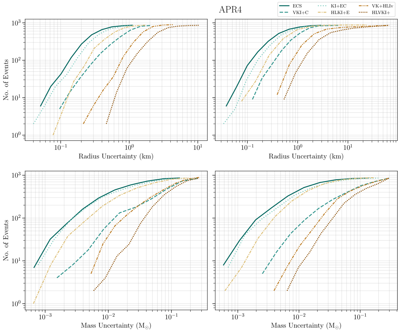
FIG. 9. Upper Panel : Cumulative histograms of the uncertainty in neutron star radii in km (top two panels) and masses in solar mass (bottom two panels) multiplied by the total number (860) of neutron stars in the 430 selected BNS events. The left panels are for events with the best measured tidal deformability and the right panels are for events with the highest SNRs. The different curves correspond to different detector networks considered in this study. These plots show that even the inclusion of just one XG detector (VKI+C or HLKI+E) leads to a vast improvement in the precision of radii measurements. Such detectors could measure the radius to within about 200 m for several events. A network containing two or three XG detectors would improve by a factor of a few. On the other hand, companion masses are better measured by a network that has ET ( 0.01 M_{\odot} to 0.001 M_{\odot} ) whose lower frequency performance helps in more accurate determination of the chirp mass and the mass ratio.
