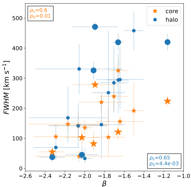
Fig. 11: FWHM of the Ly \alpha line in the core (orange stars) and in the halo (blue points) plotted against the UV continuum slope of the host galaxy (calculated in H17). The larger symbols indicate the six S/N_{\text{HALO}} > 10 objects. The Spearman rank correlation coefficients \rho_s and corresponding p_0 values are indicated. See also Fig. A.3 for other relations between the Ly \alpha line properties and the UV properties of the host galaxy.
