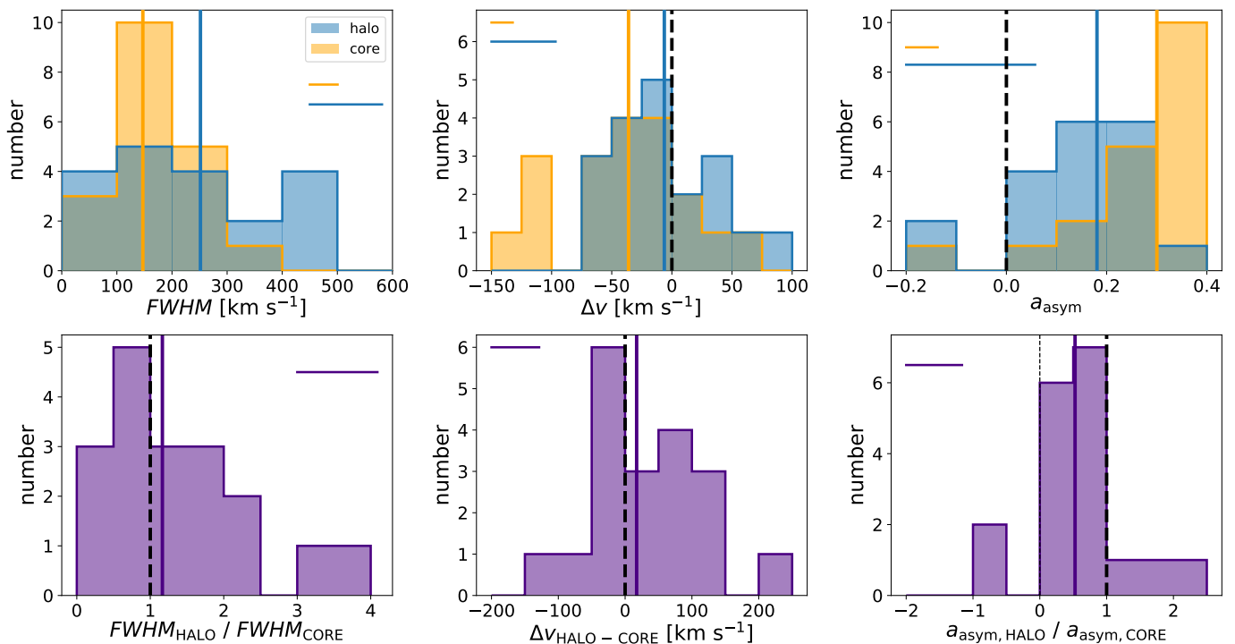
Fig. 6: Distributions of the best-fit parameters in the halo (blue) and core (orange) components (top) and their ratio or difference (bottom). The median values are indicated by the vertical solid lines. The typical errors (median values) are indicated by the horizontal solid lines in each panel. Left : Distributions of the FWHM parameters. The median values for the core, halo and ratio are 147 \text{ km s}^{-1} , 252 \text{ km s}^{-1} and 1.16 , respectively. Middle : Distributions of peak positions in the core and halo component relative to the peak of the total Ly \alpha line (top) and halo/core peak separation (bottom). The median values are -36 \text{ km s}^{-1} , -6 \text{ km s}^{-1} and +17 \text{ km s}^{-1} , respectively. Right : Distributions of the asymmetry parameters. The median values for the core, halo and ratio are 0.30 , 0.18 , and 0.5 , respectively. For visibility, the object (#7159) with halo/core FWHM ratio of 8.2 and a_{\text{asym}} ratio of -19.2 is not shown here.
