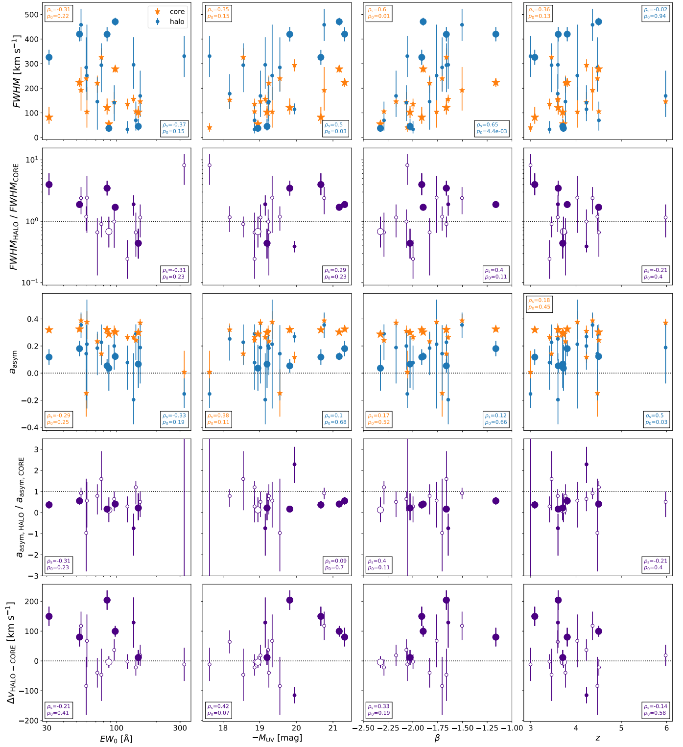
Fig. A.3: Ly \alpha emission spectral properties (same as Fig. A.2) plotted against, from left to right : the Ly \alpha EW_0 , the absolute UV magnitude, the UV continuum slope and the redshift of the host galaxy. The larger symbols indicate the six S/N_{HALO} > 10 objects. Spearman rank correlation coefficients \rho_s and corresponding p_0 values are indicated. Open circles represent the objects for which the core/halo Ly \alpha lines are not statistically different (see Sect. 5.4).
