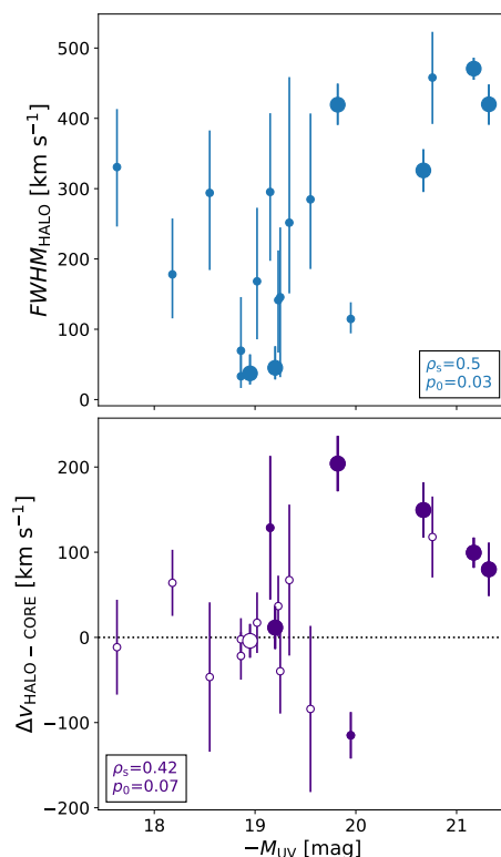
Fig. 10: Ly \alpha halo spectral properties in terms of FWHM (top) and peak shift relative to the central line (bottom) plotted against the absolute UV magnitude of the host galaxy. The larger symbols indicate the six S/N_{\text{HALO}} > 10 objects. Spearman rank correlation coefficients \rho_s and corresponding p_0 values are indicated. Open circles (bottom) represent the objects for which the core/halo Ly \alpha lines are not statistically different (see Sect. 5.4). See also Fig. A.3 for other relations between the Ly \alpha line properties and the UV properties of the host galaxy.
