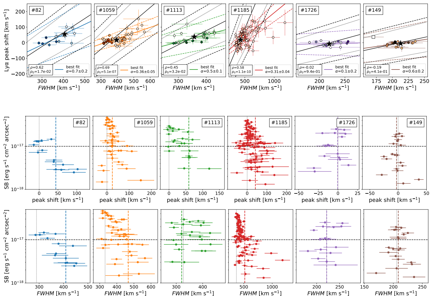
Fig. 3: \text{Ly}\alpha haloes spectral analysis of the six galaxies presented in Fig. 2. Top row : Peak velocity shift relative to the central \text{Ly}\alpha line ( r < 0''.4 ) plotted against the FWHM of the \text{Ly}\alpha lines extracted in the different Voronoi bins for the six tested objects (MUSE IDs are indicated). The brightness of the points indicates the bin surface brightness (darker point meaning higher SB). Pearson correlation coefficients \rho and corresponding p_0 values are shown in each panel. The solid colored line indicates the best fit of our data, while the dashed colored lines show the 1\sigma errors (the slope \alpha and its error are indicated in the legend). The square point (last panel) is discarded for the fit (sigma clipping factor of 4). The parameters measured on the total \text{Ly}\alpha lines are indicated by the star symbols. For comparison the re-scaled V18 relation (solid line) and its dispersion (dotted lines) are plotted in black. The black dashed lines show the V18 relation 1\sigma errors by taking into account the errors of the re-scaling procedure (see Sect. 3.3.2). Bottom rows : \text{Ly}\alpha surface brightness of the bins as a function of the peak velocity shift (top) and FWHM (bottom) of the \text{Ly}\alpha line for the six tested objects. The black dotted vertical lines indicate the central \text{Ly}\alpha line values. The black horizontal dashed line represents the arbitrary SB threshold at 10^{-17} \text{ erg s}^{-1} \text{ cm}^{-2} \text{ arcsec}^{-2} . The colored vertical dashed lines show the median values of the SB < 10^{-17} \text{ erg s}^{-1} \text{ cm}^{-2} \text{ arcsec}^{-2} bins.
