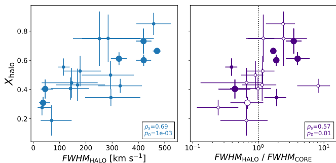
Fig. 9: Halo flux fraction plotted against the FWHM of the line in the halo (left) and halo/core FWHM ratio (right). The larger symbols indicate the six S/N_{\text{HALO}} > 10 objects. Spearman rank correlation coefficients \rho_s and corresponding p_0 values are shown in each panel. Open circles represent the objects for which the core/halo Ly \alpha lines are not statistically different in terms of width, peak position and asymmetry parameter (see Sect. 5.4). See also Fig. A.2 for the relations between the spatial and spectral properties of the LAHs.
