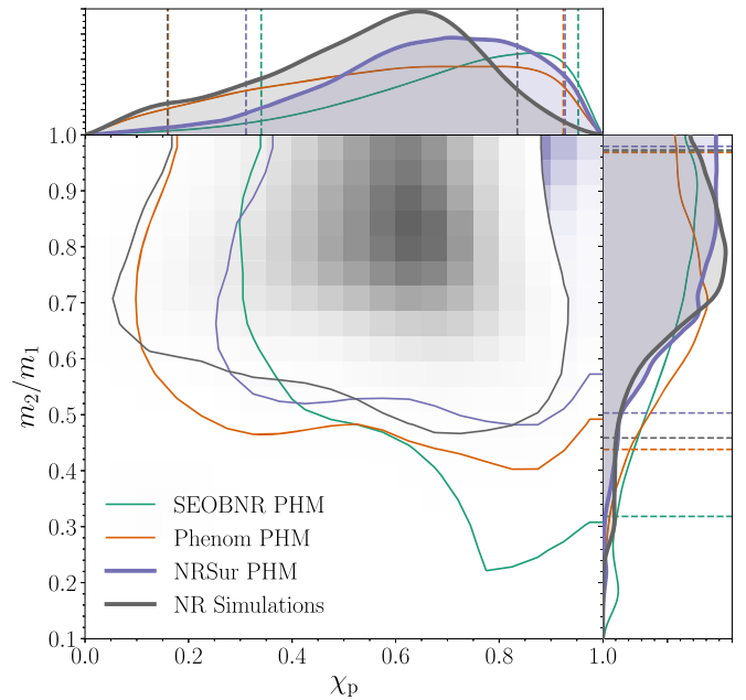
Figure 8. Posterior probability density for the precession spin parameter \chi_p and mass ratio from the direct comparison of NR simulations with GW190521 (gray tiles, and gray contour showing 90% confidence area). For comparison, shown here are the 90% bounds on these parameters from the three waveform models.
