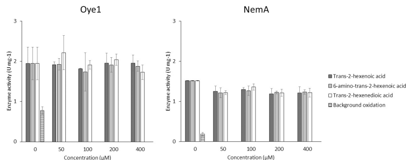
Fig 9. Inhibition test. Activity of NemaA and Oye1 in the presence of trans -2-hexenoic acid, 6-amino- trans -2-hexenoic acid, and trans -2-hexenedioic acid investigated for their inhibitory effect at concentrations up to 400 \mu M. Results are given as mean \pm standard deviation of three replicates.
