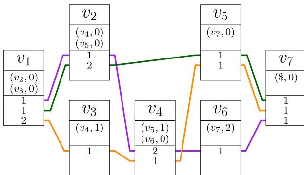
Fig. 12 The GBWT in Example 2. As in Fig. 11, the top part of each record is the vertex identifier v . The middle part stores a pair (w, BWT.rank(C[v], w)) for each outgoing edge (v, w) . The bottom part is BWT_v encoded using edge ranks
