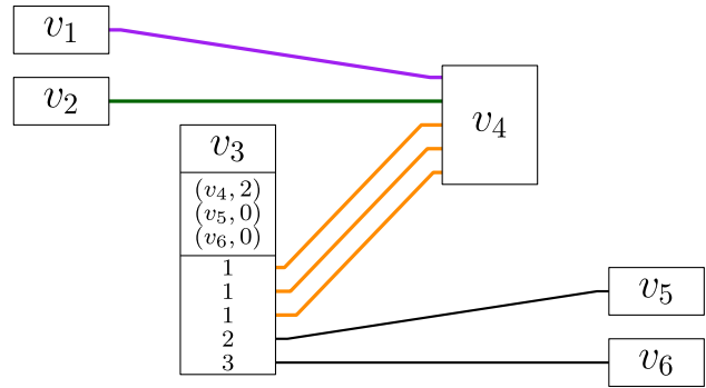
Fig. 11 The record for vertex v_3 with outgoing paths to v_4 , v_5 , and v_6 . The top part of the record is the vertex identifier. The middle part stores a pair (w, BWT.rank(C[v], w)) for each outgoing edge (v, w) . The bottom part is BWT_v encoded using edge ranks. Observe that there are two paths visiting vertex v_4 from vertices smaller than v_3 . Hence, record for vertex v_3 stores the pair (v_4, 2)
