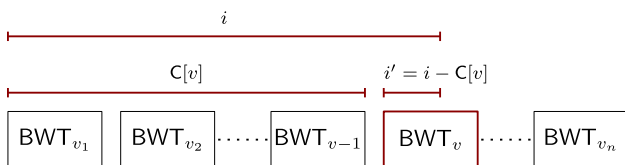
Fig. 10 Partitioning the BWT into substrings BWT_v corresponding to vertices v \in V and the representation of BWT offsets i as pairs (v, i')
