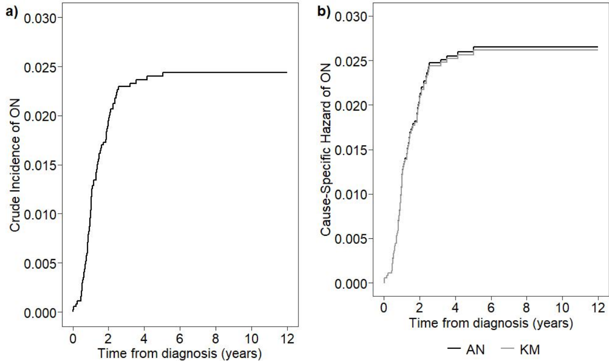
Figure 4.1: a) CI_{ON}(t) estimated through the Aalen-Johansen formula; b) AN_{ON}(t) and KM_{ON}(t) smoothed curves of the CSH_{ON}(t) .
