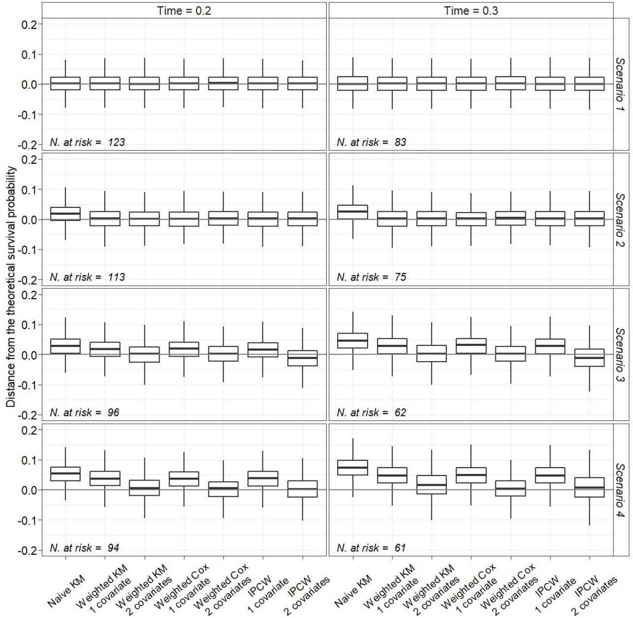
Figure 6.1: Simulation results in all scenarios at times t = 0.2 and t = 0.3 . The grey horizontal line is the reference null bias.
