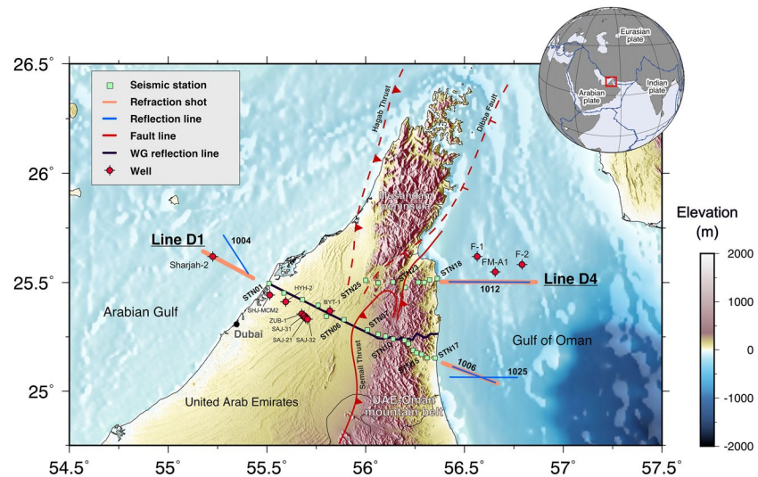
Figure 1. Location map of the study area. Green squares are the broadband seismometers used in the experiment. Stations are progressively counted from west to east along Line D1 (STN01–STN17) and from east to west along Line D4 (STN18–STN25). Colored lines offshore the UAE show multichannel-seismic profiles (blue lines) and wide-angle reflection and refraction profiles (orange lines) acquired by R/V Hawk Explorer. The main tectonic structures are highlighted with red lines. Location of the wells are taken from WesternGeco Report (2005). The inset in the upper right corner shows the location of the UAE along with the main plate boundaries in blue.
