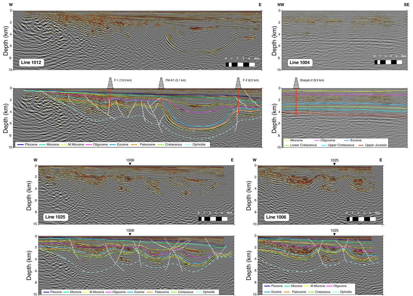
Figure 2. Pre-stack depth-migrated images. Lines 1012 and 1006 are coincident with the eastern offshore portions of Line D4 and D1, respectively. Colored lines mark prominent reflectors and interpreted stratigraphy tied to well F-1, FM-A1 and F-2 (red vertical lines). White lines are interpreted faults (positive flower structure). Colored horizons are dashed where uncertain. Location of the seismic transects is shown in Figure 1.
