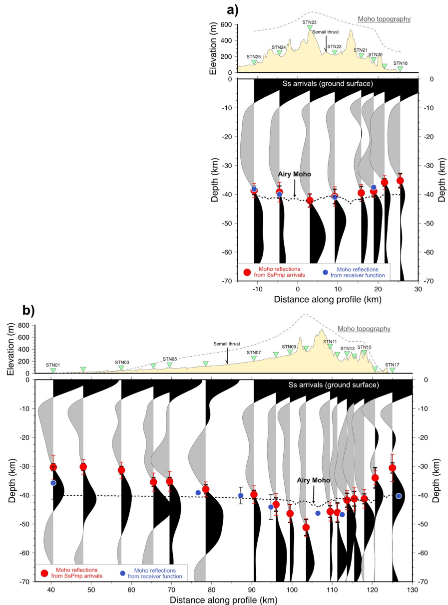
Figure 7. Depth-migrated 1-D reflection profiles constructed using the SsPmp phase. (a) Line D4; (b) Line D1. Red dots are the estimated crustal-thickness values with relative uncertainties obtained through bootstrapping displayed as vertical red bars. Thick, black error bars associated with red dots are uncertainties derived by depth migrating the VDSS traces assuming a \pm 0.1 km/s perturbation of the bulk V_p . For comparison, receiver-function-derived crustal depths (Ali et al., 2020) are included as blue dots. Topography is shown above each profile. Black dashed lines show the expected depth-to-Moho assuming an Airy model of isostasy. Gray dashed lines above the topography plots show the smoothed, inverted, seismically constrained Moho to highlight a possible lateral offset between the topographic peak and the crustal root (D1). The offset is not readily visible along Line D4, perhaps due to the fact that our station coverage across the transition from mountain belt to foreland area is more limited.
