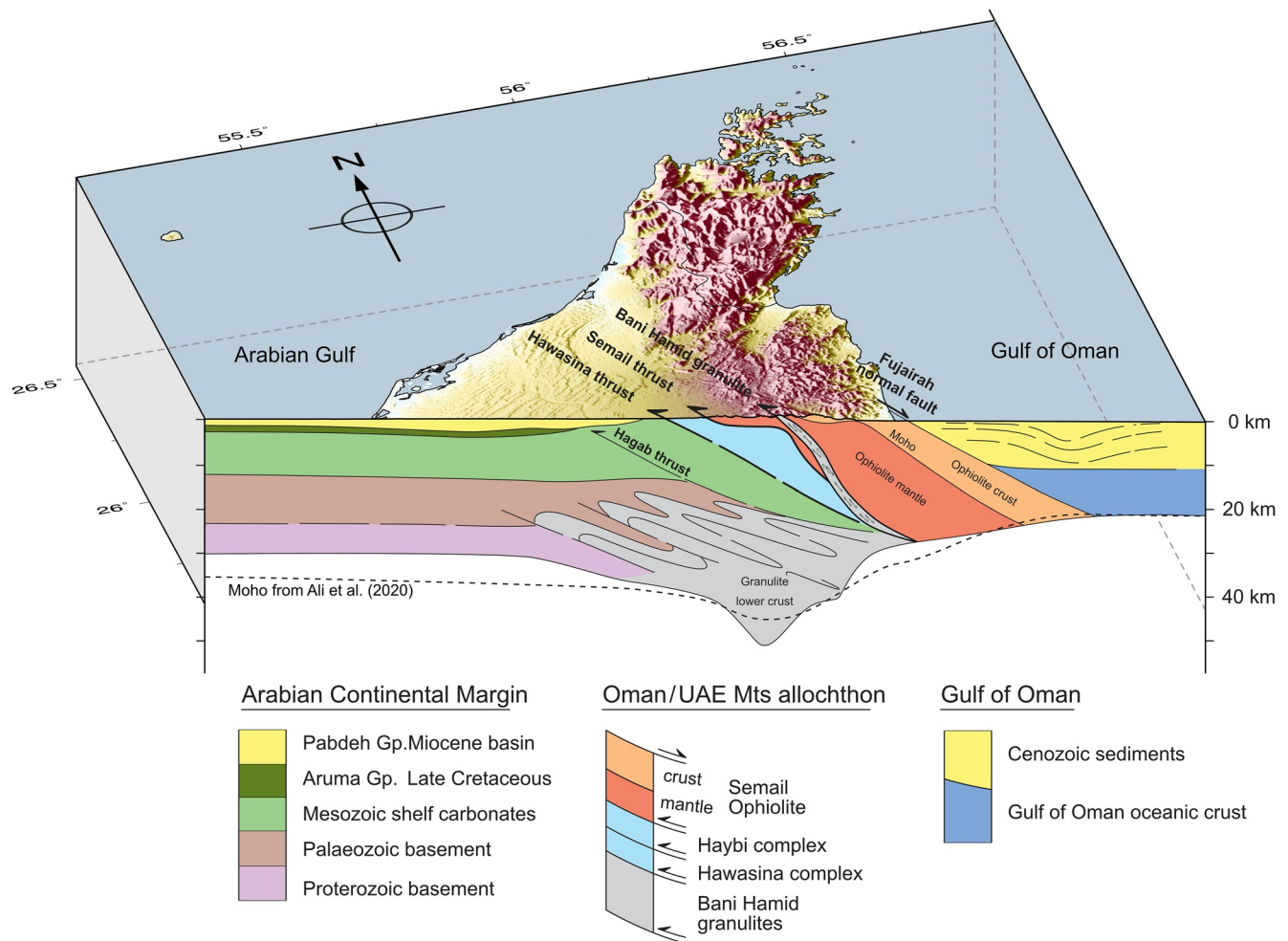
Figure 9. Conceptual geological interpretation of a cross section across the UAE-Oman mountains and its bounding sedimentary basins. Our interpretation is consistent with the results obtained in this study and in Ali et al. (2020). Dashed-black line is Moho depth from Ali et al. (2020).
