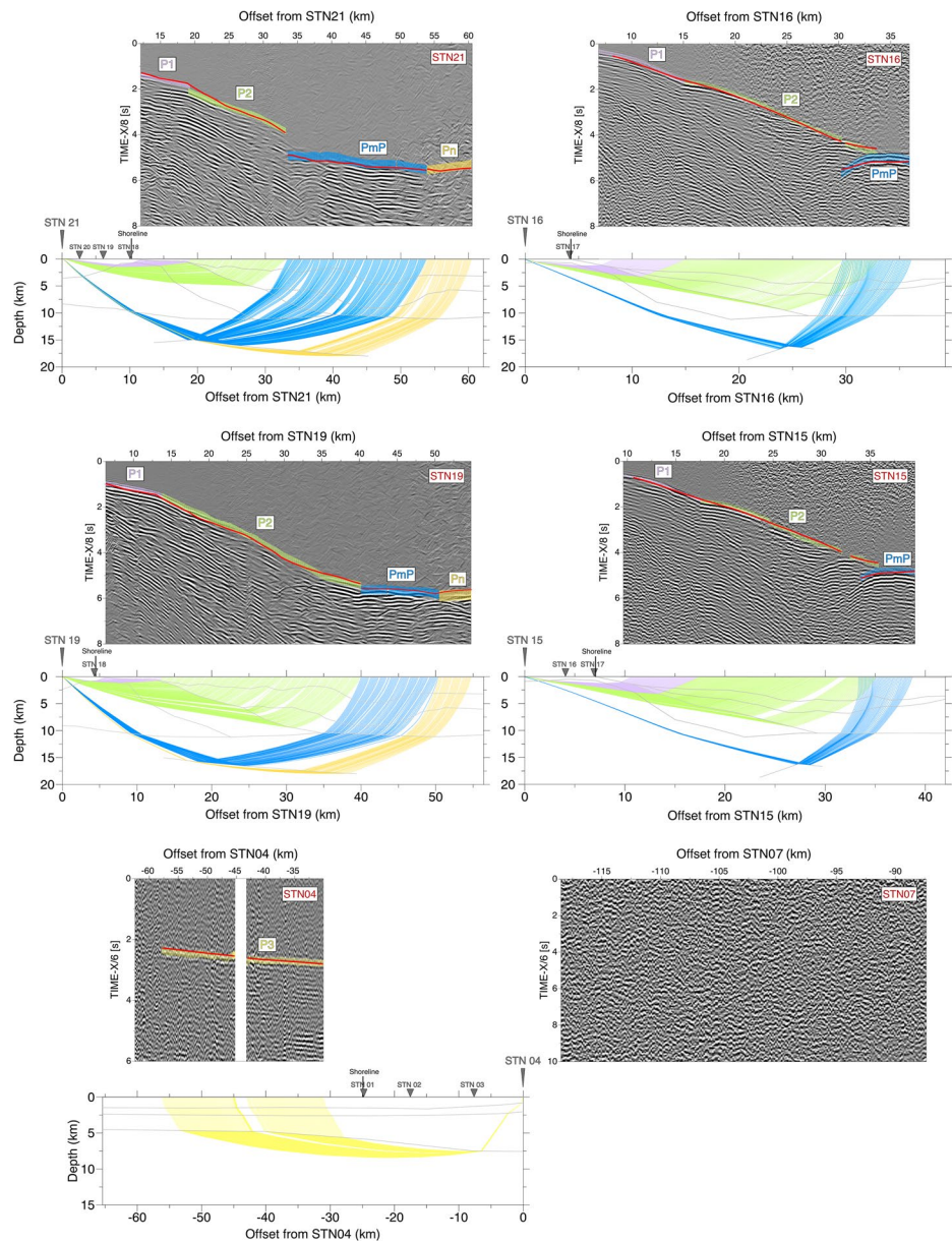
Figure 3. Representative record sections for receiver gathers STN15, STN16, STN19, STN21, STN04, and STN07. Records from STN15 and STN19 have been modified from Ali et al. (2020). Receiver gathers display the identified seismic phases (colored lines) and predicted travel times based on the final model shown in Figure 6 (red dots). Receiver gathers are underlain by corresponding ray path plots. STN07 did not record usable data from the sources located in the Arabian Gulf.
