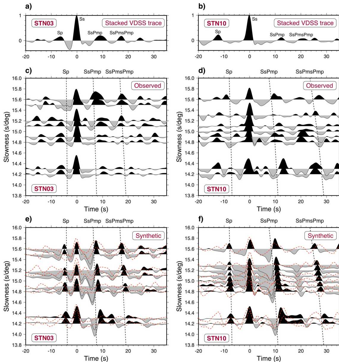
Figure 5. Two examples of observed (c), (d) and synthetic traces (e), (f) for STN03 and STN10. (a) and (b) are obtained by stacking all available VDSS traces for the respective station. Traces are aligned along the Ss arrival at time zero. The dashed black lines are the predicted traveltimes for Sp , SsPmp and SsPmsPmp phases, calculated using a modified version of the ak135 velocity model to include the crustal thickness estimated with the 1-D migration procedure. Clear moveout of the SsPmp phase is observed across the slowness range, arriving earlier at large slowness (i.e., shorter epicentral distance). Note the larger arrival time of the SsPmp phase that characterizes STN10, compatible with a greater crustal thickness. Dashed red lines in (e) and (f) are VDSS observed traces that overly the synthetic seismograms.
