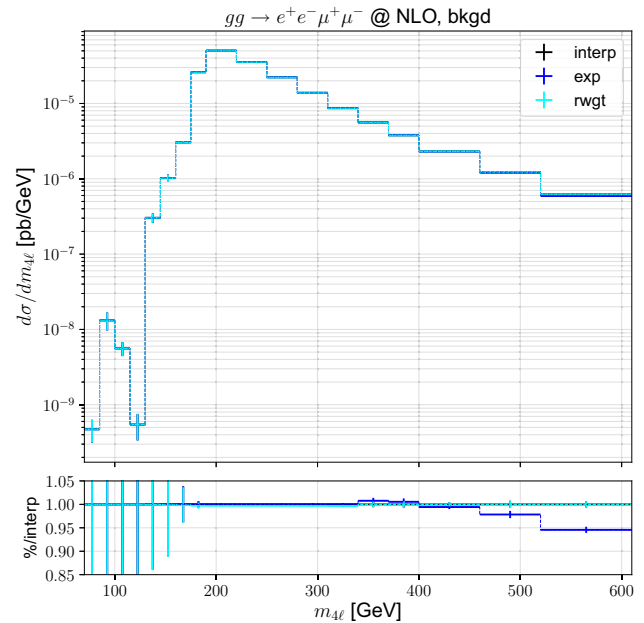
Fig. 14 Differential distribution in invariant mass m_{4\ell} of the four-lepton system in gg \rightarrow e^+e^-\mu^+\mu^- at fixed-order NLO for the background contribution. The upper panel shows nominal predictions obtained using different approximations for the two-loop amplitude: 1/m_t expansion (exp, blue), reweighting with the exact one-loop amplitude (rwgt, cyan), and an interpolation between the two options (interp, black). The ratio plot shows the relative yield of the different contributions with respect to the interpolated results
