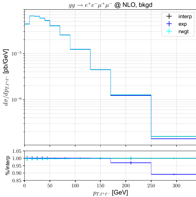
Fig. 15 Differential distribution in transverse momentum p_{T, \ell^+ \ell^-} of the dilepton system \ell^+ \ell^- = e^+ e^-, \mu^+ \mu^- in gg \rightarrow e^+ e^- \mu^+ \mu^- at fixed-order NLO for the background contribution. Predictions and colour coding are as in Fig. 14
