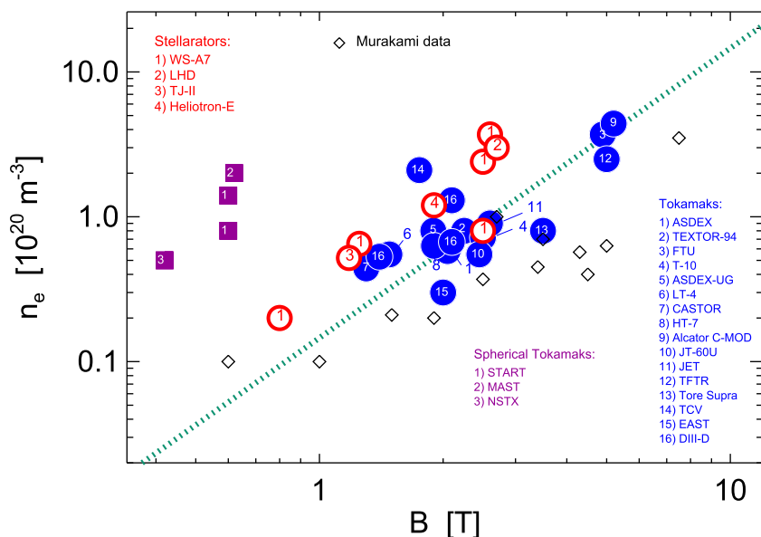
FIG. 1. Density limit values vs B for various machines: conventional tokamaks, for which recent data are shown (see Refs. 32–47) along with the original ones of Murakami (see Ref. 31), stellarator machines, 48–51 and spherical tokamaks. 52–54 Dotted line is the theoretical density limit (11).
