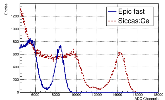
Fig. 2. Light output spectra of the Epic fast and Siccas Cerium-doped sample. The crystal with only Ce-doping shows the highest light output, whilst the stabilization of \text{Ce}^{4+} centres speeds up scintillation at the expense of light output.
