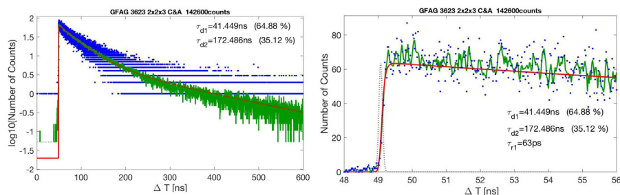
Fig. 3. TCSPC measurement of the GFAG 2 × 2 × 3 mm 3 sample. Blue dots are the measured entries, the red solid line the fitting curve, and the green solid line is a running average of the blue data points as a guide for the eye. The IRF of the system is shown as a black dotted line. Left: log scale plot, highlighting the decay. Right: zoom on the rising edge. (For interpretation of the references to colour in this figure legend, the reader is referred to the web version of this article.)
