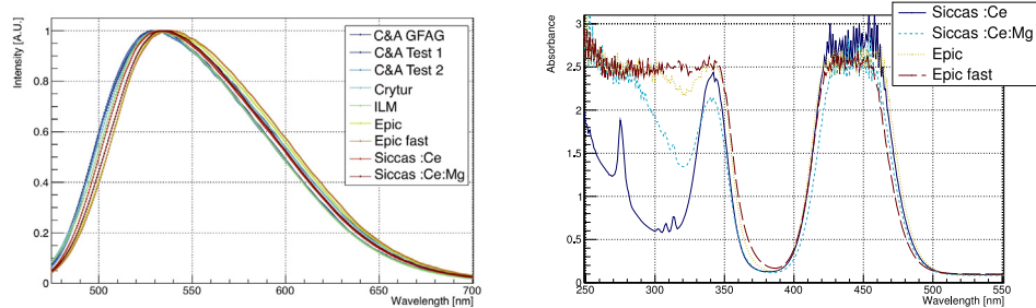
Fig. 1. Left: Photoluminescence emission spectra of all the 2 \times 2 \times 3 \text{ mm}^3 samples tested. The spectra span 470 to 700 nm, all peaking in the 520–540 nm range. Right: Absorbance spectra of four typical 2 \times 2 \times 3 \text{ mm}^3 samples. They differ mainly below 350 nm: whilst the solely Cerium-doped Siccas shows Gd-related transition peaks, stabilization of \text{Ce}^{4+} increases absorption.
