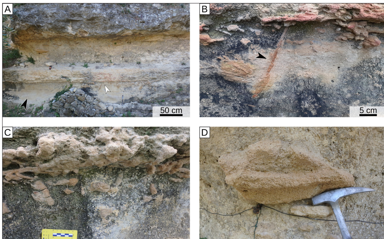
Fig. 8 - Section S5. A) Overview of the section showing a Glossifungites ichnofacies (white arrowhead) carved into the underlying layer (black arrowhead). B) Detail of the Glossifungites ichnofacies with a long Skolithos shaft (black arrowhead). C) Detail of the Thalassinoides burrows. D) Detail of the breccia layer including large angular clasts of coarse-grained Pliocene calcarenites.
