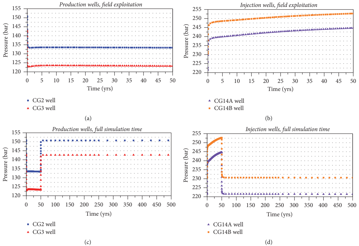
FIGURE 8: Evolution of well pressures during the exploitation process simulation at 2 selected production (CG2 and CG3, see Figure 1) and 2 injection (CG14A and CG14B, see Figure 1) wells: (a) and (b) refer to the 50-year simulation time and (c) and (d) to the 10,000-year recovering time. The initial 500 years are shown in the full simulation time plots ((c) and (d)) as full recovery is reached. This allows better visualization of the transition between the field exploitation and the quick reestablishment of the initial undisturbed pressures.
