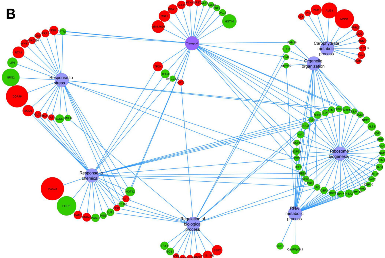
Figure 6. The comparative transcriptomic profile of CDR6/ROA1 null mutant NKKY101. A , the genes with \geq 2 -fold change are annotated on the basis of biological processes using CGD Go-slim mapper. The x axis indicates the biological functional categories, and the y axis indicates the number of genes. Left column , categories of genes that are only up-regulated; middle column , categories of genes that are up- and down-regulated; right column , the categories of genes that are only down-regulated. B , interaction map of the CDR6/ROA1 null mutant NKKY101 using five major categories from up- and down-regulated genes. Clustering was based on gene involvement in biological functions using Cytoscape software. Red and green circles , genes down- and up-regulating, respectively. The size of the circle is proportional to -fold change (the higher the -fold change, the bigger the size of the circle).
