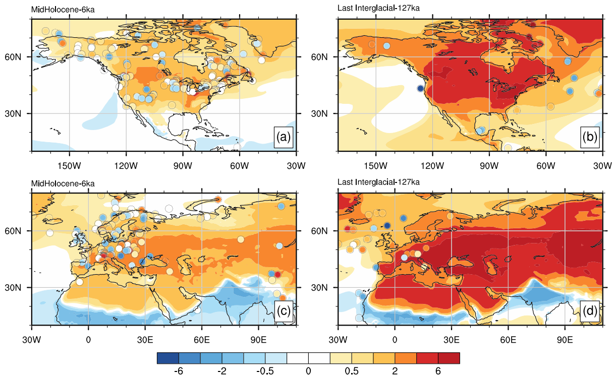
Figure 13. JJA surface air temperature anomalies ( ^{\circ}\text{C} ) in the lig127k (right) and midHolocene (left) simulations as compared to proxy reconstructions. See Kaufman et al. (2020) and Otto-Bliesner et al. (2020) for details of proxy reconstructions.
