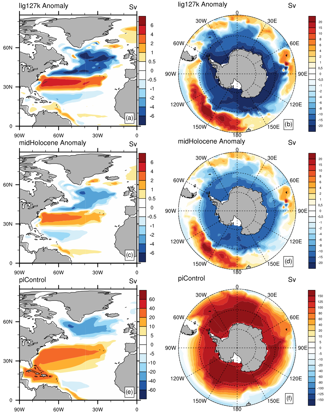
Figure 8. Anomalies of annual mean barotropic streamfunction (BSF) for the lig127k (top), midHolocene (middle) as compared to the mean BSF in the piControl (bottom) simulations for the North Atlantic (left) and the Southern Ocean (right) basins. Positive (negative) streamlines denote clockwise (counterclockwise) circulation and anomalies, such that anomalies of the same (opposite) sign as the piControl BSF suggest strengthened (weakened) circulation. Note the change in contour interval between upper and lower, and left and right panels.
