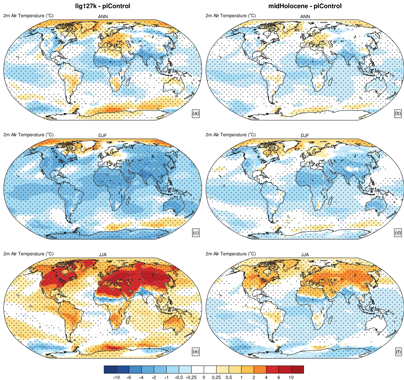
Figure 3. Annual and seasonal surface air temperature anomalies ( ^{\circ}\text{C} ) in the lig127k and midHolocene simulations as compared to the piControl simulation. Stippling indicates anomalies statistically significant at 95% level.
