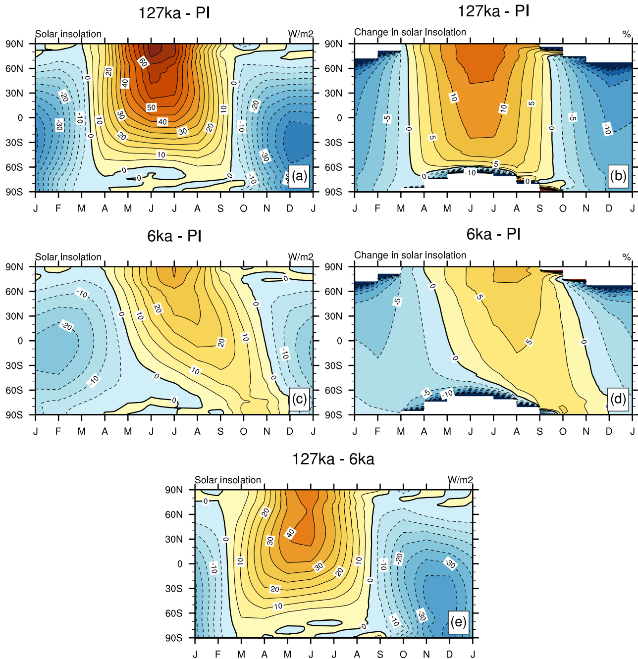
Figure 1. Seasonal cycle of insolation anomalies for the midHolocene and lig127k simulations. a), c), e) W m^{-2} ; b), d) percentage change from the piControl .
