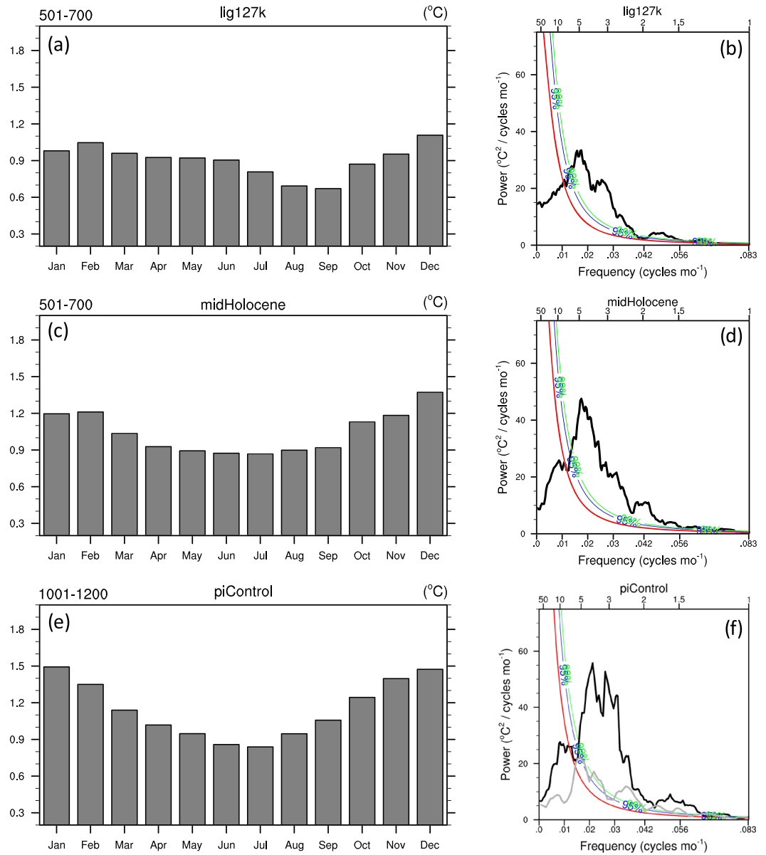
Figure 10. The monthly standard deviations ( ^{\circ}\text{C} ) and power spectra ( ^{\circ}\text{C}^2/\text{cycles mo}^{-1} ) of Niño3.4 SST in the lig127k , midHolocene , and piControl simulations. The mean annual cycle is removed prior to every calculation by subtracting the long-term monthly means. The best-fit first-order Markov red noise spectrum (red curve) and its 95% (blue curve) and 99% (green curve) confidence bounds are shown for the power spectra. The observed power spectra for 1920–2018 from the HadISST dataset is shown in light gray in panel f).
