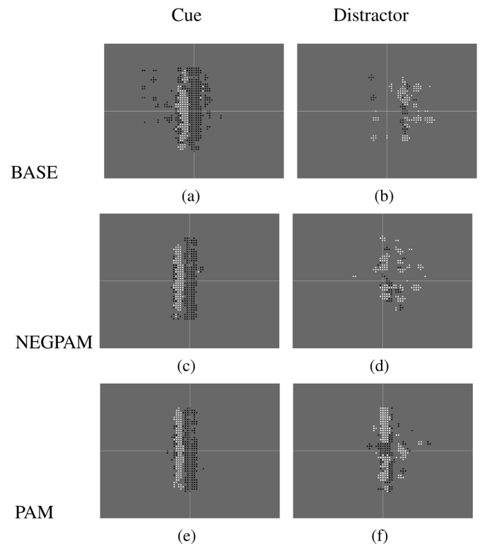
Fig. 13. Vote map of the BASE (a,b), NEG-PAM (c,d), and PAM (e,f) systems after learning, when they foveate a cue (a,c,e) or a distractor (b,d,f). Data plotted as in Fig. 8.
