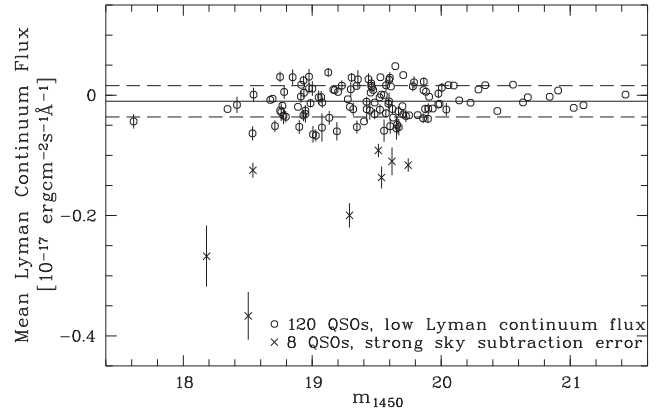
Figure 3. Mean Lyman continuum flux of the 128 quasars of our sample with a likely optically thick LLS versus their apparent AB magnitude at \lambda_r = 1450 \text{ \AA} . Error bars are the standard error of the mean flux. Error bars smaller than the symbol size are not plotted. Crosses indicate the eight quasars affected by systematic sky subtraction errors (significantly negative flux). The solid and dashed lines mark the average ( -1 \times 10^{-19} \text{ erg cm}^{-2} \text{ s}^{-1} \text{ \AA}^{-1} ) and the standard deviation ( 2.6 \times 10^{-19} \text{ erg cm}^{-2} \text{ s}^{-1} \text{ \AA}^{-1} ), of the 120 remaining measurements, respectively.
