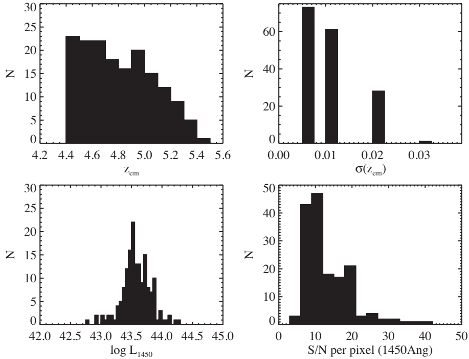
Figure 1. Histograms summarizing properties of the quasars and their spectra from the GGG survey ( top left: quasar redshift; top right: estimated redshift error; bottom left: specific luminosity at rest-frame wavelength \lambda_r = 1450 \text{\AA} ; bottom right: S/N per pixel at \lambda_r = 1450 \text{\AA} ). The sample is restricted to quasars with z_{\text{em}} > 4.4 and, given the magnitude limit of SDSS, comprise a very luminous cohort ( L_{1450} \gtrsim 10^{43} \text{ erg s}^{-1} \text{\AA}^{-1} ).
