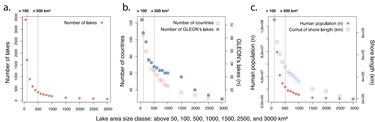
Fig. 3. Effect of different size classes on the spatial distribution and abundance of large lakes in the world. a. Number of lakes by lake size class, b. number of countries and GLEON's lakes by size class (Sharma et al., 2015), and c. sum of shore length and number of human population by size class of lakes. Note the exponential increase in the number of countries and humans affected by lake services as we include lakes of smaller size.
