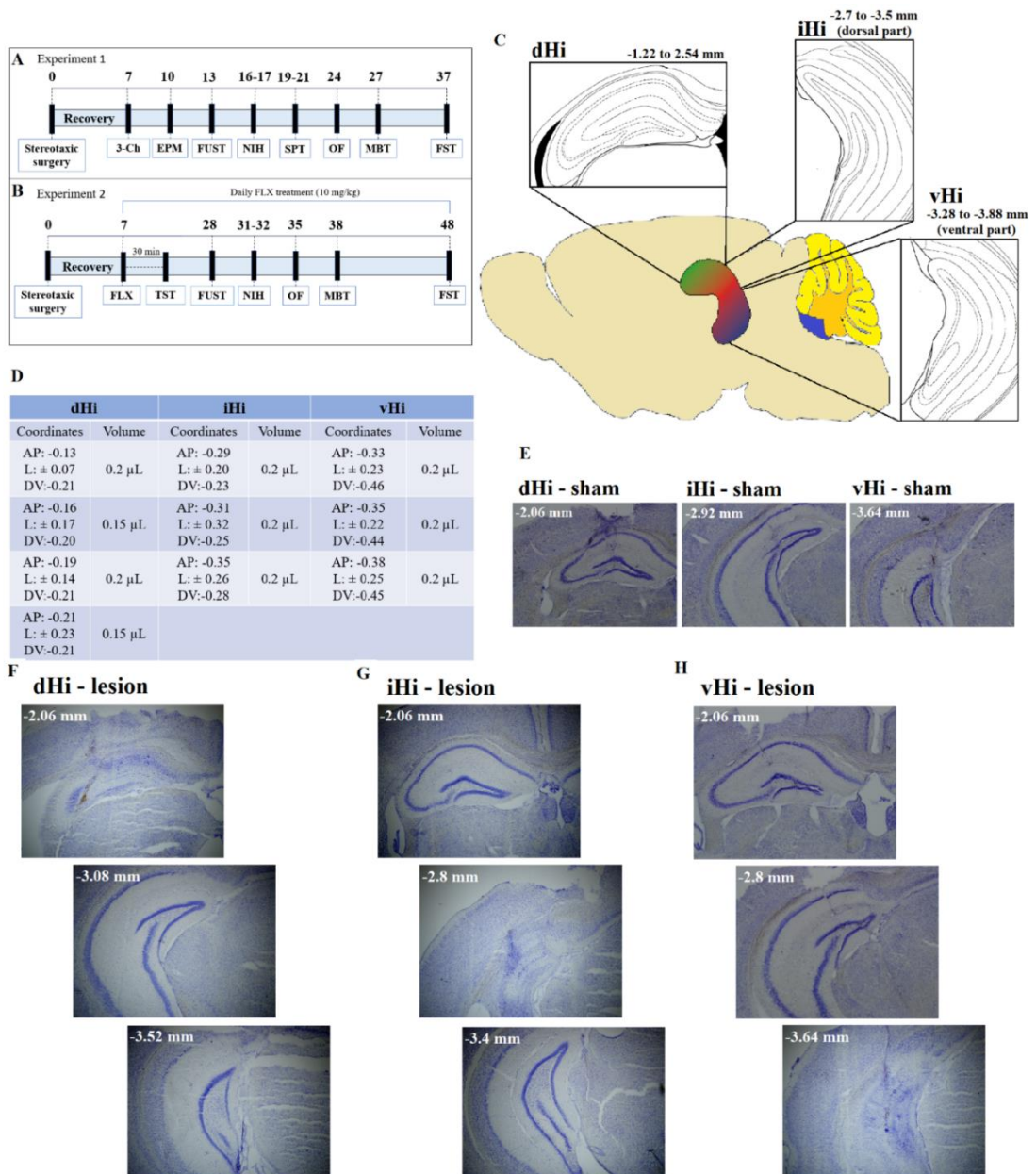
Figure 2.1: Dorsal (dHi), intermediate (iHi) or ventral (vHi) hippocampus were lesioned and animals followed with a battery of behavioural testing with or without chronic treatment with fluoxetine. A , schematic of the experiment in which animals had their dHi, iHi or vHi lesioned and followed with a battery of behavioural testing under baseline. In B , after surgery, animals followed with a battery of behavioural and neuroendocrine testing under chronic fluoxetine treatment. C , illustration of the definitions and coordinates of dHi, iHi and vHi. D , stereotaxic coordinates used to lesion dHi, iHi and vHi, bilaterally. E-H , representative images of the dHi, iHi and vHi. Lesions were confirmed using cresyl violet staining, E , dHi, iHi and vHi sham groups. F , dHi lesion, showing that iHi and vHi were intact. G , iHi lesion, showing that dHi and iHi were intact. H , vHi lesion, showing that dHi and iHi were intact. Coordinates in the representative images are in relation to bregma. Abbreviations: 3-Ch: three-chambers test, AP: anteroposterior, DV: dorsoventral, EPM: elevated plus maze, FLX: fluoxetine, FST: forced swim test, FUST: female urine sniffing test, L: lateral, MBT: marble burying test, NIH: novelty-induced hypophagia, OF: open field, SPT: saccharin preference test, TST: tail suspension test.
