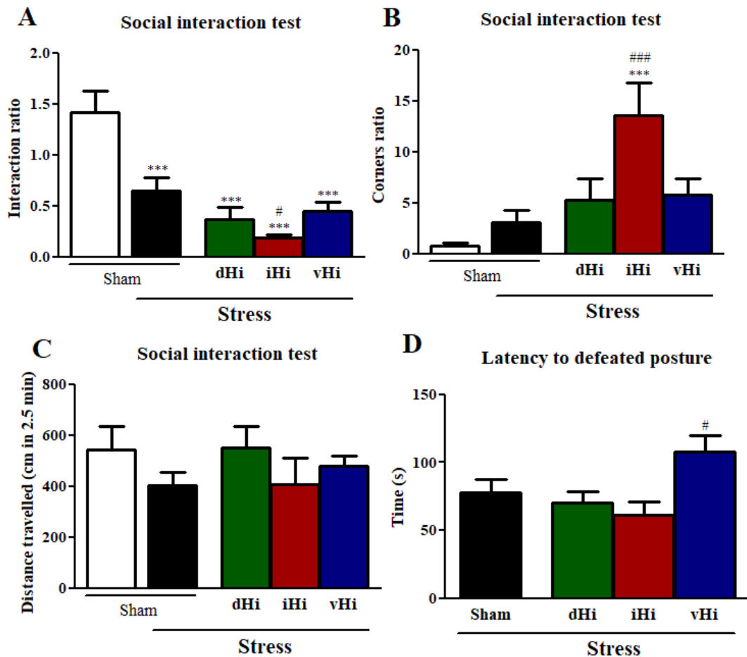
Figure 3.3: Social interaction test and latency to assume defeated posture. A , stress induces social avoidance, reducing interaction ratio. B , iHi lesion increases social avoidance, increasing corners ratio. C , stress and/or hippocampal lesions did not alter exploration of the social interaction chamber. D , average latency to assume a defeated posture in the first social defeat session is increased in vHi -lesioned animals. * p < 0.05 , *** p < 0.001 , in relation to sham-no stress group; # p < 0.05 , ### p < 0.001 , in relation to sham-stress group, according to Fishers LSD post-hoc test.
