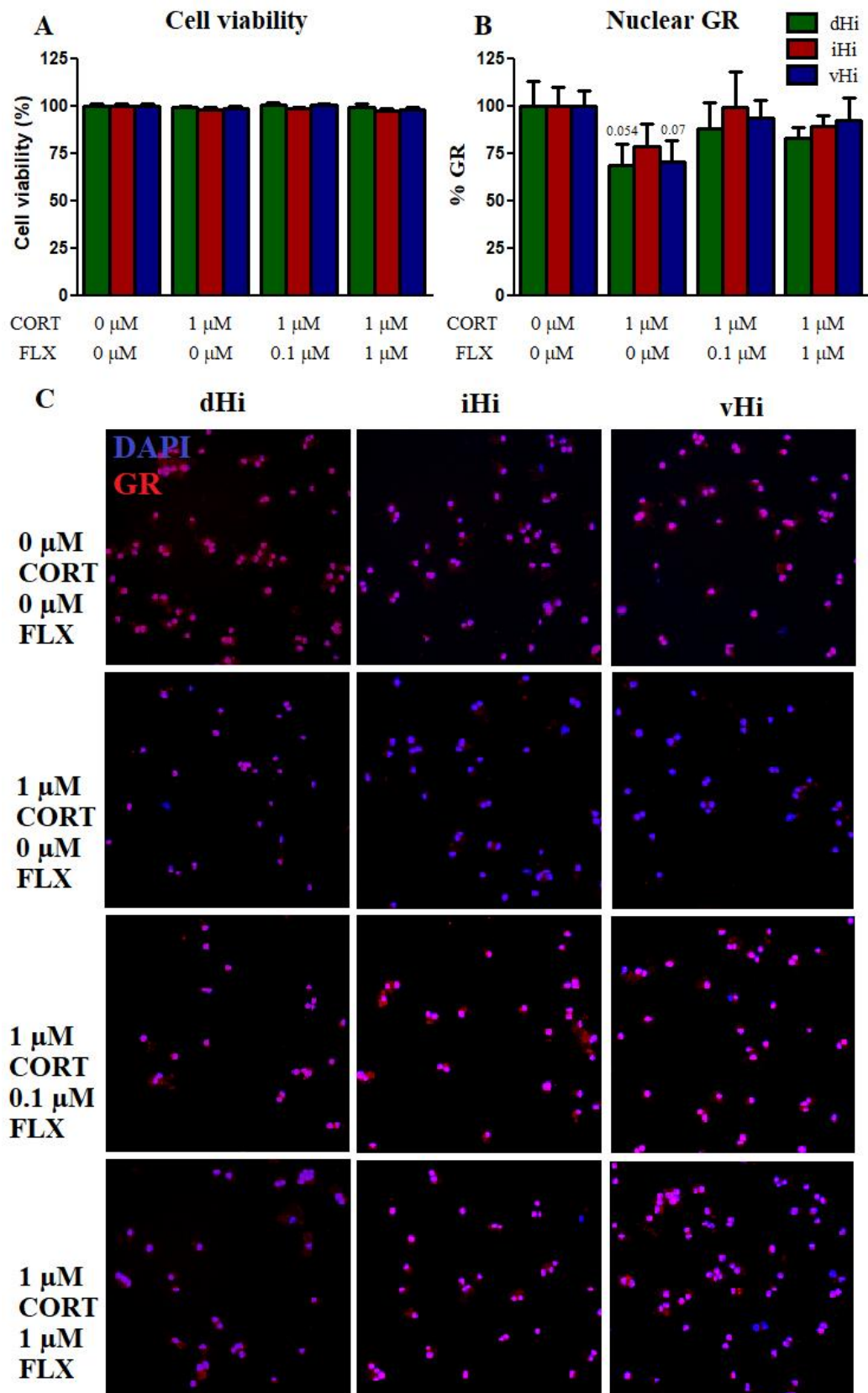
Figure 5.5: Effects of fluoxetine and corticosterone on cell viability and nuclear GR expression. A, Neither corticosterone alone nor corticosterone plus fluoxetine co-treatment affected cell viability as assessed with an MTT assay. B, Fluoxetine seems to alleviate corticosterone-induced reductions on nuclear GR expression irrespective of the hippocampal sub-region cells were derived from. C, representative images of cells derived from the dHi, iHi and vHi stained with DAPI (blue) and GR (red).
