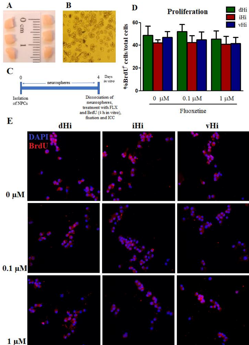
Figure 5.1: Effects of acute fluoxetine exposure (4 h in vitro) on cell proliferation from NPCs derived from dHi, iHi and vHi. A, dHi, iHi and vHi dissected from P28 Sprague-Dawley rats. B, NPCs growing as neurospheres. C, Experimental timeline: NPCs were isolated and cultured as neurospheres for 4 DIV, then dissociated and treated with fluoxetine (0.1 \mu M or 1 \mu M) for 4h in vitro prior to fixation and immunocytochemistry. D, Fluoxetine did not affect cell proliferation (BrdU + cells) in NPCs derived from the dHi, iHi or vHi. E, Representative images of proliferating cells derived from the dHi, iHi and vHi; stained with DAPI (blue) and BrdU (red).
