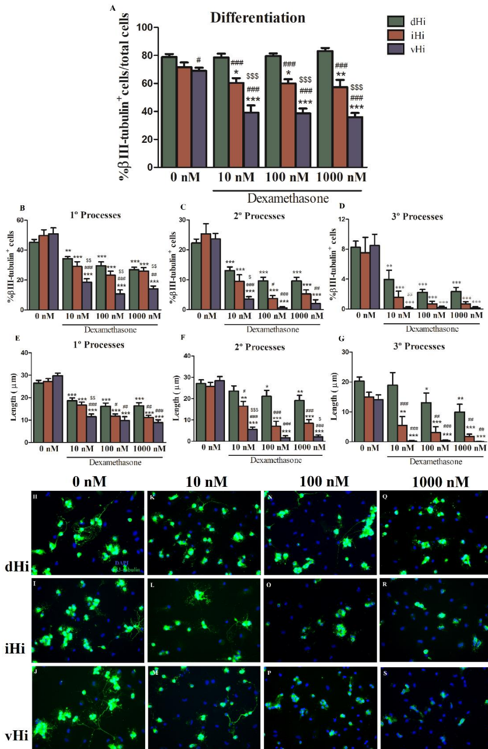
Figure 4.4: Effects of long-term dexamethasone exposure on NPCs differentiation into neurons ( \beta 3 -tubulin + ) and their maturation. A , dexamethasone reduces neuronal differentiation, specifically on cells derived from the iHi and especially from the vHi; B-G , dexamethasone reduces neuronal maturation, especially in cells derived from the vHi, reducing the percentage of \beta 3 -tubulin cells with primary ( B ), secondary ( C ) and tertiary processes ( D ) and the length of these processes ( D-F ); H-S , representative images of cells stained with DAPI (blue) and \beta 3 -tubulin (green). * p < 0.05 , ** p < 0.01 , *** p < 0.001 , compared with respective 0 nM group, # p < 0.05 , ## p < 0.01 , ### p < 0.001 , compared to cells derived from the dHi treated with the same concentration of dexamethasone, $ p < 0.05 , $$ p < 0.01 , $$$ p < 0.001 , compared to cells derived from the iHi treated with the same concentration of dexamethasone.
