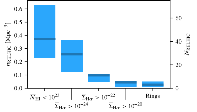
Figure 7. Number density distribution of \text{H}\alpha -fluorescent haloes in APOSTLE. The median values are shown by thick solid lines; shaded regions indicate 10 th –90 th percentiles. From left to right, we show the number density of all RELHICs with H I column densities below our star formation threshold, those with surface brightnesses exceeding three different limiting values, and those with discernible ring-shaped surface brightness profiles. Here, N_{\text{H I}} \equiv N_{\text{H I}}/(\text{cm}^2) and \Sigma_{\text{H}\alpha} \equiv \Sigma_{\text{H}\alpha}/(\text{erg s}^{-1} \text{ cm}^{-2} \text{ arcsec}^{-2}) . The right-hand axis indicates the corresponding number counts per APOSTLE volume.
