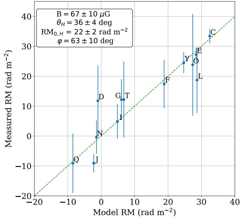
340 Fig. 4. Best fit of the RM in the Galactic wind model. The Galactic wind is assumed to follow the geometry described in the text and in Fig. 3. The plot shows the measured RM versus the RM predicted by the best fit. The best-fitting values for the parameters are shown in the box. The error bars are at 1\sigma . For a perfect fit, all points should fall on the dashed green line, which represents the identity function.
