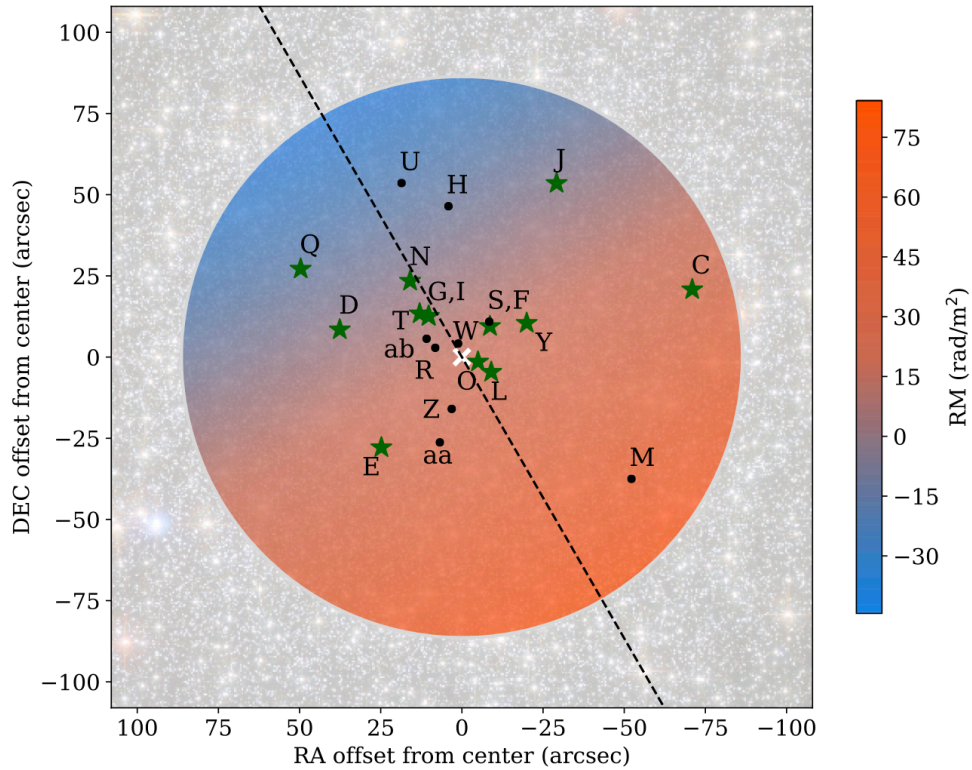
315 Fig. 2. Map showing the gradient in RM and the distribution of pulsars in 47 Tuc. The colour scale shows the RM values predicted by the best-fitting linear gradient model presented in Fig. 1. The pulsars for which a measurement of RM was possible are represented by green stars while the pulsars with no measured RM are represented by black dots. The dashed line shows the direction of the \vec{R} axis in Fig. 1. A white cross marks the optical centre of the cluster (38). 320 Credits of background image: NASA, ESA, and the Hubble Heritage (STScI/AURA)- ESA/Hubble Collaboration. Acknowledgment: J. Mack (STScI) and G. Piotto (University of Padova, Italy).
