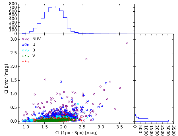
Figure 9. The measured CI and errors for all clusters in all filters in the LEGUS dwarfs. We find a median CI of 1.7 mag with a standard deviation of 0.27 mag, and a median CI error of 0.04 mag with a standard deviation of 0.12 mag.
