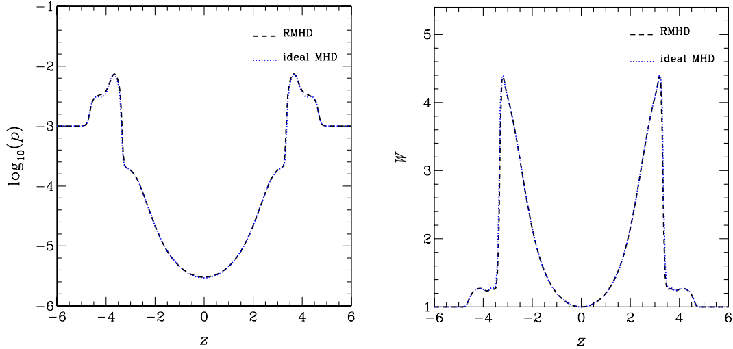
FIG. 7 (color online). Left panel: One-dimensional cuts along the z -direction and at t = 4.0 of the pressure. The black dashed line corresponds to the resistive code (the WHISKYRMHD code), while the blue dotted line corresponds to the ideal-MHD code (the WHISKYMHD code). Right panel: The same as in the left panel but for the Lorentz factor.
