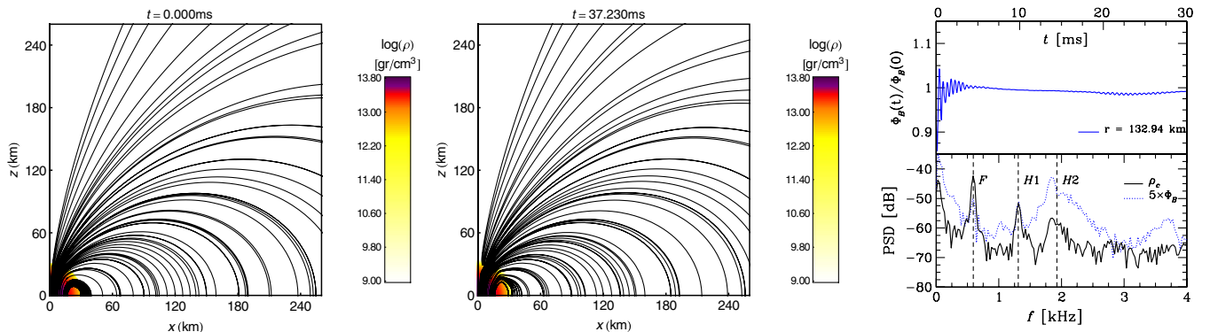
FIG. 11 (color online). Left and middle panels: Evolution of the magnetic field lines displayed at times t = 0 ms and t = 37.23 ms. The rest mass density is also shown with purple-red-yellow colors. Right panel: The top part shows the evolution of the magnetic flux computed across a hemispheric surface at a radius r = 132.94 km, while the bottom part shows the power spectral density of the rest-mass density (black solid line) and of the magnetic flux (blue dotted line).
