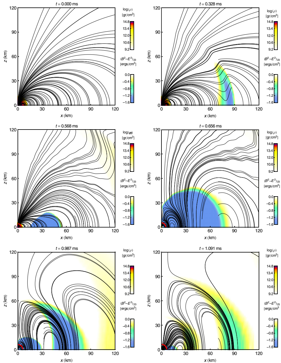
FIG. 14 (color online). The same as in Fig. 12, but where in addition to the rest-mass density (color code from white to red) and the magnetic-field lines (thin solid lines) we show the electrically-dominated regions (i.e., B^2 - E^2 < 0 , color code from light blue to white in units of 10^{23} ).
