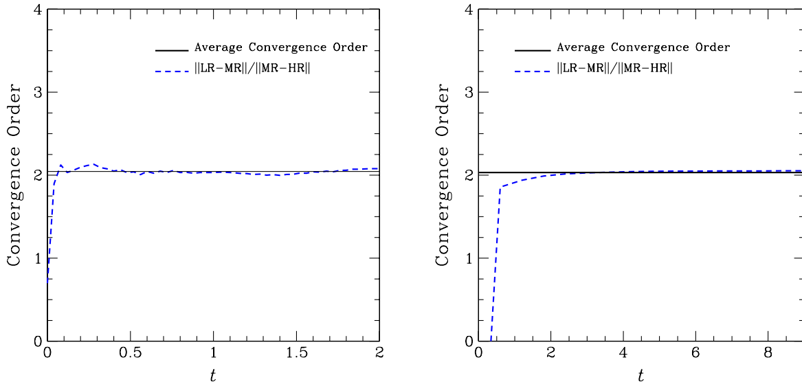
FIG. 18 (color online). Left panel: Convergence order as a function of time for the one-dimensional Alfvén-wave test we have performed in flat spacetime (Sec. IVA 1) for a uniform conductivity \sigma = 10^6 . The average convergence order is 2.05. Right panel: The same as in the left one, but for the one-dimensional current-sheet test in Sec. IVA 2 for a uniform conductivity \sigma = 100 . The average convergence order is 2.03.
