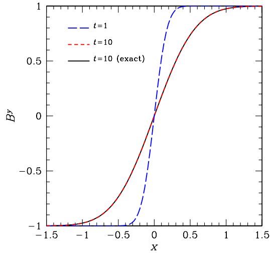
FIG. 2 (color online). Self-similar current sheet. B^y component of the magnetic field at the initial t = 1 and final time t = 10 . The exact solution at t = 1 is shown with a dashed blue line. The solution given by the analytic expression (48) at t = 10 (black solid line) is indistinguishable from the numerical solution obtained from the resistive MHD equations (red dashed line).
