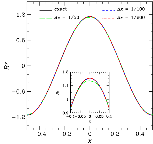
FIG. 1 (color online). Circularly polarized Alfvén wave. B^y component of the magnetic field for three different resolutions \Delta x = \{1/50, 1/100, 1/200\} , together with the exact initial solution (black solid line). Clearly, the numerical solution provided by the resistive MHD implementation and the exact one overlap for a uniform conductivity \sigma = 10^6 and the highest resolution.
