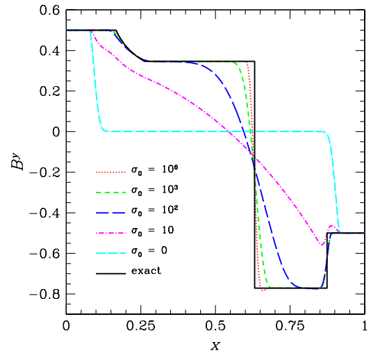
FIG. 4 (color online). Shock-tube tests. B^y component of the magnetic field for conductivities \sigma_0 = \{0, 10, 10^2, 10^3, 10^6\} at t = 0.4 and resolution \Delta x = 1/200 . For \sigma_0 = 0 the magnetic field is governed by a wavelike equation, corresponding to the solution of the Maxwell equations in vacuum.
