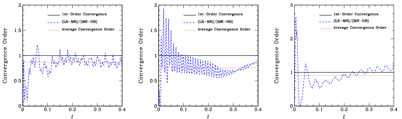
FIG. 19 (color online). Convergence Tests. We report the convergence order as a function of time for the one-dimensional shocktube tests we have performed in flat spacetime (Sec. IVA 3) for \sigma = 10^6 , \sigma = 10 and for a nonuniform power-law conductivity with \sigma_0 = 10^6 and \gamma = 9 , respectively. The convergence order as given by taking the average of the convergence order over time for these three different tests (from left to right) is 0.87, 0.76, 0.91, respectively.
