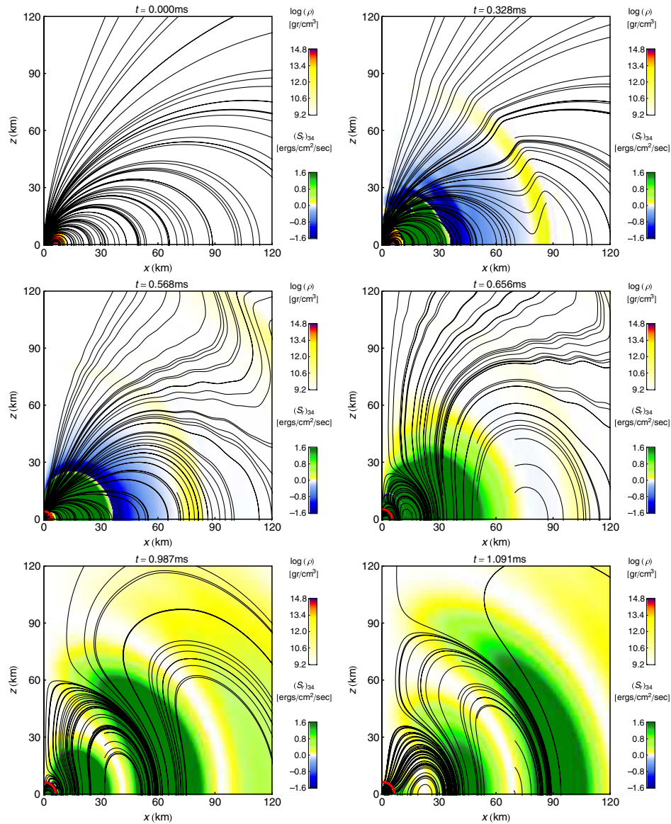
FIG. 12 (color online). Two-dimensional cuts on the (x, z) plane of the collapse to a BH of a magnetized NS. Shown with colors are the rest-mass density (color code from white to red) and the radial Poynting vector (color code from blue to green) in units of 10^{34} , while thin lines reproduce the magnetic-field lines. The different snapshots refer to times t = 0, 0.32, 0.57, 0.65, 1.0 and 1.1 ms, and an apparent horizon is marked with a thin red line starting from t = 0.57 ms. Note that all the matter is accreted into the hole and that a quadrupolar QNM ringdown is clearly visible in the Poynting flux.
