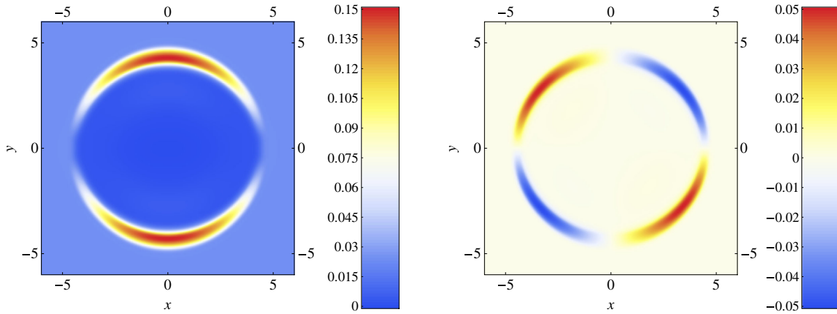
FIG. 6 (color online). Left panel: Snapshot of the magnetic field component B^y in the (x, y) plane at t = 4.0 ; Right panel: Snapshot of the magnetic field component B^y in the (x, y) plane at t = 4.0 .
