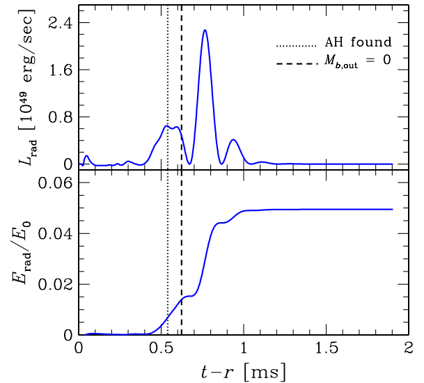
FIG. 15 (color online). Top panel: Luminosity calculated at a distance r = 88.63 km from the compact object. The black dotted line represents the time at which the apparent horizon is formed and the black dashed line corresponds to the time at which all the matter is well within the horizon. Bottom panel: Evolution of the total radiated energy normalized to the initial magnetic energy.
