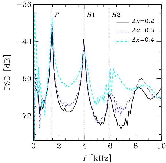
FIG. 9 (color online). Power spectral density of a full general-relativistic evolution of the central rest-mass density for a stable star with confined magnetic fields. Different line types refer to different resolutions. Shown with dotted vertical lines are the eigenfrequencies obtained from linear perturbation theory.
