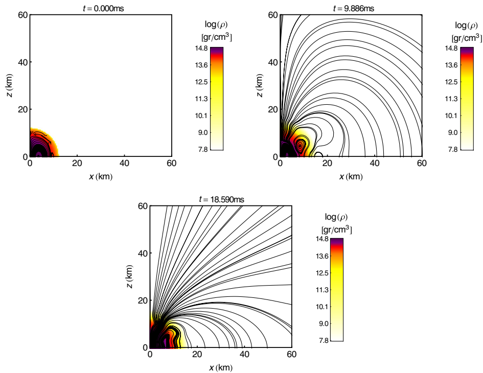
FIG. 10 (color online). Two-dimensional cuts on the (x, z) plane of the solution of the rest-mass density (color code from white to red) and the magnetic field lines at times t = 0, 9.88, and 18.59 ms. The evolution refers to a nonrotating star in a dynamical spacetime. Note that although the magnetic field is contained in the star initially, it diffuses out as a result of numerical and physical resistivity.
