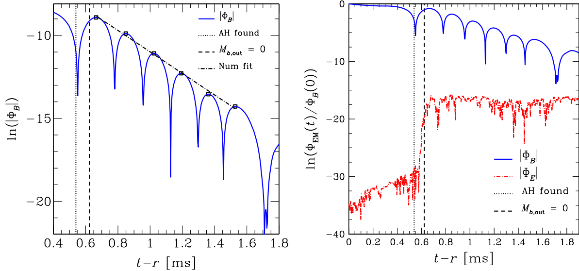
FIG. 16 (color online). Left panel: QNM ringdown of the magnetic field as measured through the magnetic flux at r = 36.93 km. Again, the black dotted line represents the time at which the apparent horizon is formed and the black dashed line corresponds to the time at which all the matter is well within the horizon; the dot-dashed line represents instead our fit to an exponential decay. Right panel: Logarithm of the absolute values of the magnetic and electric fluxes as normalized to the initial magnetic flux.
