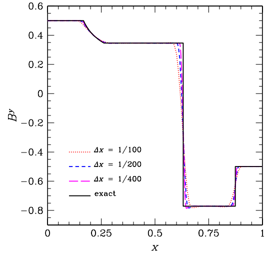
FIG. 3 (color online). Shock-tube tests. B^y component of the magnetic field at t = 0.4 for different resolutions \Delta x = \{1/100, 1/200, 1/400\} . The highest resolution \Delta x = 1/400 matches the exact ideal-MHD solution remarkably well.
