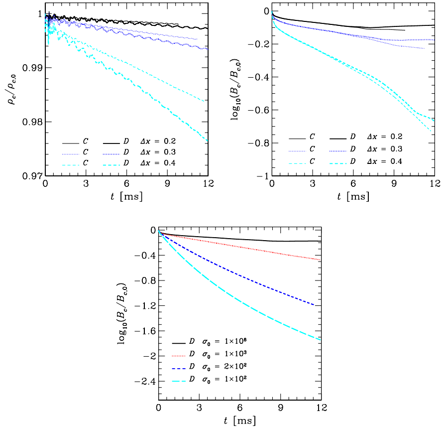
FIG. 8 (color online). Left panel: Evolution of the central rest-mass density of a nonrotating magnetized star for both the Cowling approximation (C, thin lines) and a dynamical spacetime (D, thick lines). Different line types mark different resolutions: dashed light blue \Delta x = 0.443 km, dotted dark blue \Delta x = 0.295 km, continuous black \Delta x = 0.222 km. Middle panel: The same as the left one but for the central magnetic field. Right panel: The same as the middle one but different values of the conductivity \sigma_0 . All lines refer to a resolution of \Delta x = 0.222 km.
