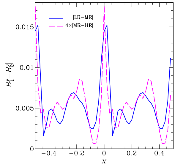
FIG. 17 (color online). Convergence tests. Absolute errors of the solution of the y component of the magnetic field B^y along x for different resolutions rescaled by a factor of four (as dictated by our scheme) regarding the one-dimensional Alfvén-wave test we have performed in flat spacetime (Sec. IVA 1) for a uniform conductivity \sigma = 10^6 .
