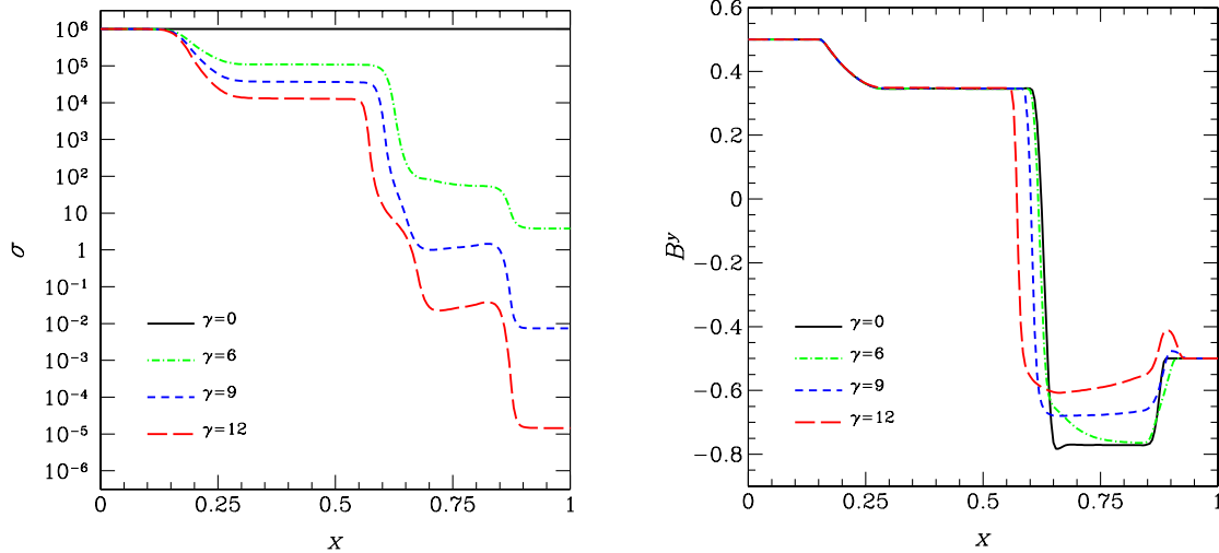
FIG. 5 (color online). Shock-tube tests. The left panel shows the conductivity profile at t = 0.4 for nonuniform conductivity with different power laws, i.e., \gamma = \{0, 6, 9, 12\} . The \gamma = 0 case corresponds to the high-conductivity regime of the resistive MHD equations. The right panel reports instead the B^y component of magnetic field for the same initial conditions as in the left one. The leftmost region tends to the ideal MHD solution, while the rightmost tends to the vacuum solution for \gamma = 12 .
