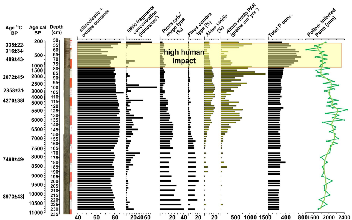
Fig. 3 - Fossil Alnus viridis PAR data and pollen inferred annual precipitation from Armentarga fossil record compared with other palaeoecological and geochemical data.
