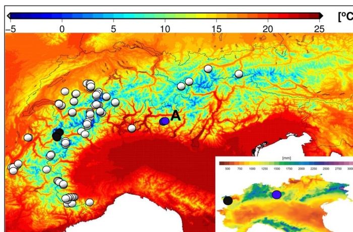
Fig. 1 - Map of July climatology (1961-1990) with 170 EMPD sites (white dots), La Thuile Valley training set (black dots), Upper Brembana Valley training set (blue dots) and Armentarga fossil site (A) plotted. On the right map of annual precipitation (1961-1990) and the location of the two altitudinal training sets
