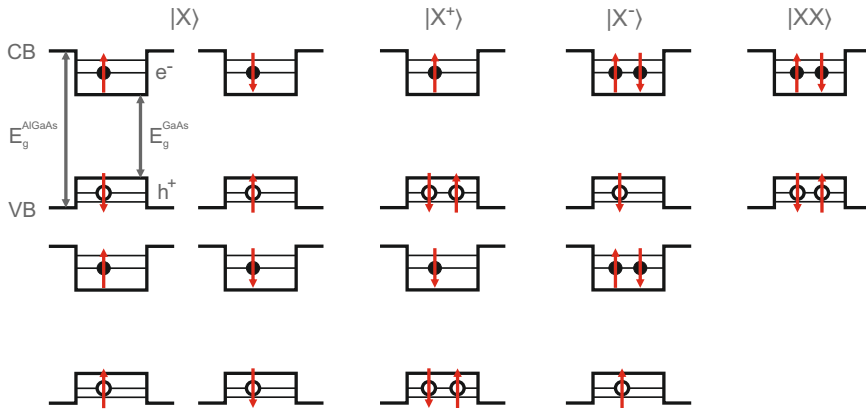
FIGURE 3.2: Possible spin configurations of the neutral exciton (X), the singly charged excitons (positive X^+ and negative X^- ) and the biexciton (XX) in the s-shell of a GaAs/AlGaAs quantum dot.
