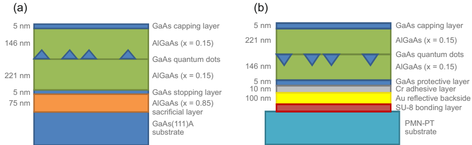
FIGURE 6.1: a) Structure of a sample with sacrificial layer and barrier thickness adjusted for a metal-semiconductor-air cavity. b) Structure of the processed sample after transfer of the active semiconductor membrane on a piezoelectric substrate.
