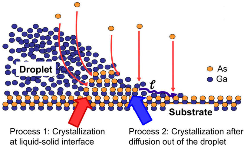
FIGURE 3.6: The diagram outlines the two competing mechanisms which lead to As incorporation. Image taken from Ref. [29].
