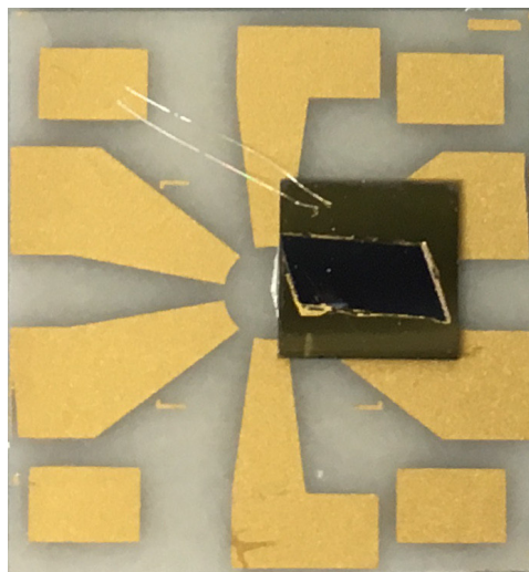
FIGURE 6.8: Picture of a semiconductor membrane containing quantum dots transferred on a piezoelectric substrate mounted on a chip carrier.
