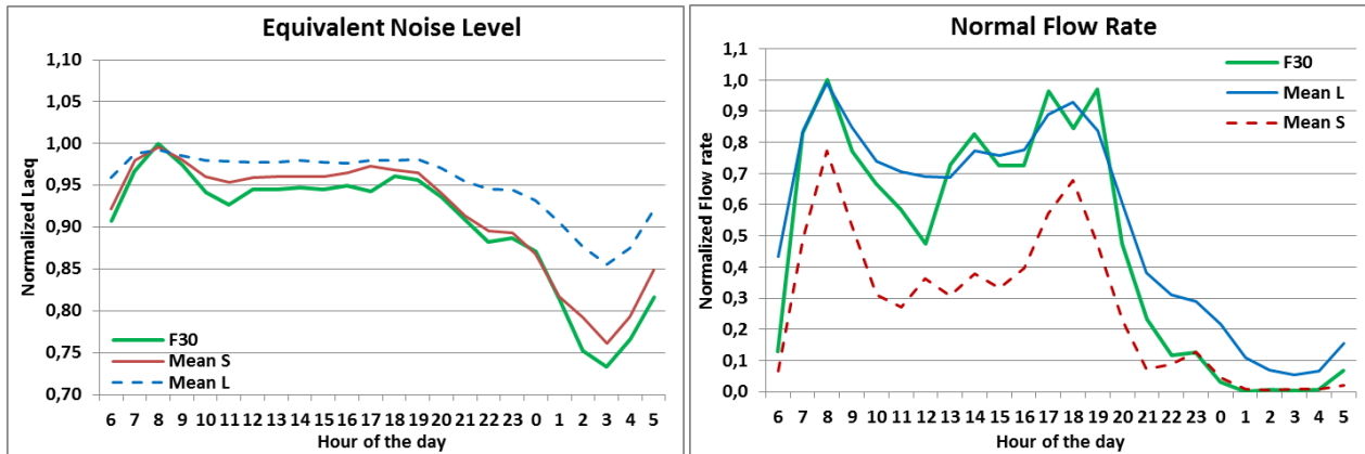
Figure 3: Example of stretch (F30) which belongs to the ‘small’ cluster for noise while included in the ‘large’ cluster from the flow rate analysis. (Left panel) Equivalent noise level results for road F30. As shown, F30 belongs to the small cluster (Cluster 2). (Right panel) Traffic flow rate for F30 showing that it belongs to the large cluster (Cluster 1). In both cases, the continuous lines for the mean values correspond to the cluster at which F30 belongs to, while the dashed lines display the result for the opposite cluster.
