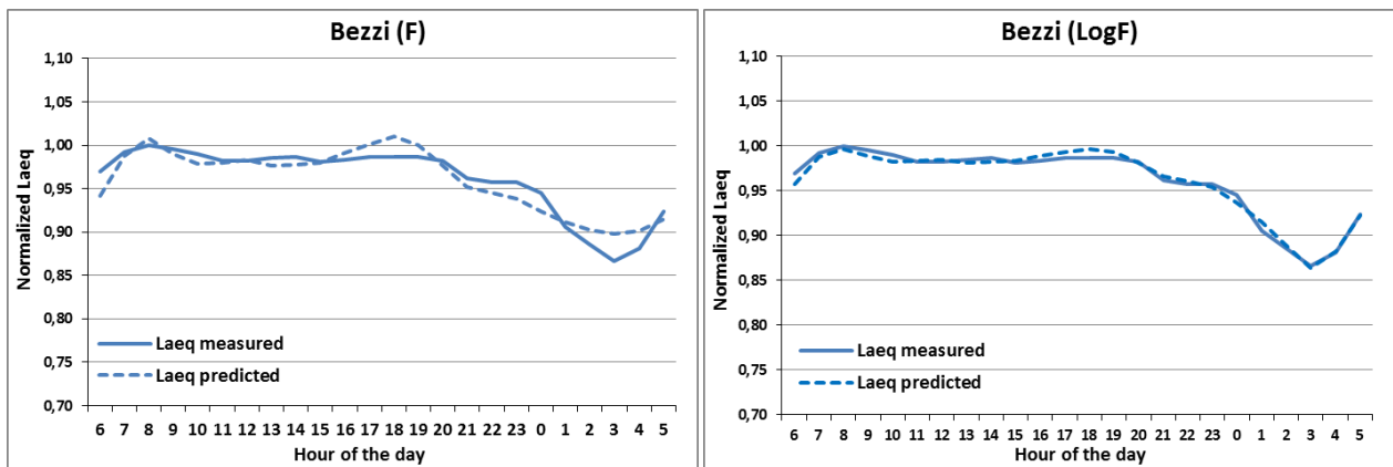
Figure 4: Fitting of the normalized equivalent level, LAeq, vs intraday hour, for the two models, Eq. (3) for F and Eq. (4) for LogF, for the street Bezzi. Least square fit parameters for: (F) \alpha = 0.118 , \beta = 0.892 , and mean square fit error \varepsilon = 0.015 (1.079 dB); (LogF) A = 0.381 , B = 0.616 , and \varepsilon_{Log} = 0.006 (0.420 dB).
