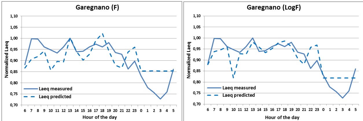
Figure 5: Fitting of the normalized equivalent level, L_{Aeq} , vs intraday hour, for the two models, Eq. (3) and Eq. (4), for a second example, street Garegnano. Least square fit parameters for: (F) \alpha = 0.168, \beta = 0.853 , and mean square fit error \varepsilon = 0.063 (3.919 dB); (LogF) A = 0.168, B = 0.818 , and \varepsilon_{Log} = 0.051 (3.175 dB).
