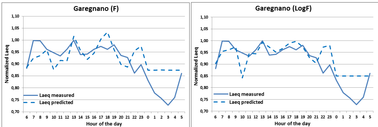
Figure 7: Fitting of the normalized equivalent level, L_{Aeq} , vs intraday hour, for the two models, Eq. (3) and Eq. (4), using the mean cluster values for the street Garegnano ( \alpha_S = 0.159, \beta_S = 0.874 ) and ( A_S = 0.148, B_S = 0.849 ), yielding mean square fits errors: \varepsilon = 0.065 (4.081 dB) (F) and \varepsilon = 0.056 (3.472 dB) (LogF).
