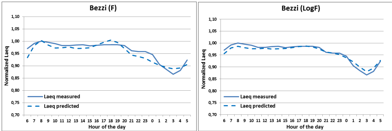
Figure 6: Fitting of the normalized equivalent level, L_{Aeq} , vs intraday hour, for the two models, Eq. (3) and Eq. (4), using the mean cluster values for the street Bezzi ( \alpha_L = 0.123, \beta_L = 0.881 ) and ( A_L = 0.309, B_L = 0.678 ), yielding mean square fits errors: \varepsilon = 0.016 (1.209 dB) (F) and \varepsilon = 0.010 (0.701 dB) (LogF).
