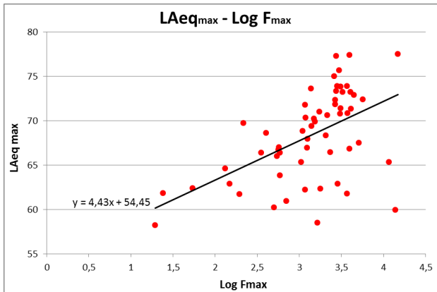
Figure 8: Plot of the maximum equivalent level, L_{Aeqmax} , vs the logarithm of the maximum flow rate, \text{Log } F_{nmax} for all the stretches considered here. The straight line is a least-square-fit with equation: y = A_{max}x + B_{max} , with A_{max} = 4.43 and B_{max} = 54.45 , yielding a mean error (standard deviation of the data from the fit) of \epsilon \approx 6\% .
