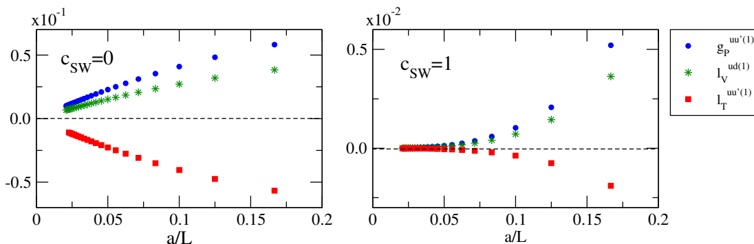
Figure 7. Vanishing P_5 -odd correlation functions at one-loop order, calculated for c_{\text{sw}} = 0 (left panel), c_{\text{sw}} = 1 (right panel) and for \theta = 0 . The series for m_{\text{cr}}^{(1)}(a/L) (5.16) and z_f^{(1)}(a/L) (5.17) have been inserted and C_F = 4/3 (note the scale difference between the panels).
