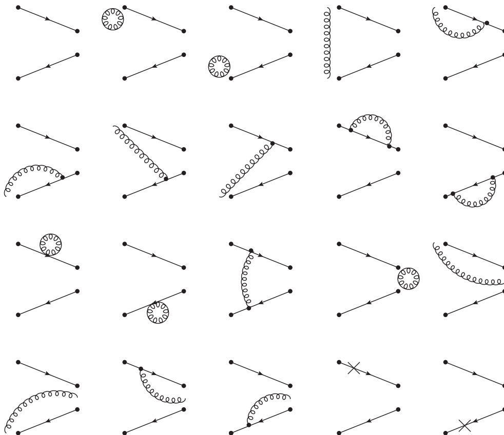
Figure 3. The set of tree-level and one-loop diagrams contributing to the boundary-to-bulk correlation functions involving the point-split vector current, i.e., g_{\bar{V}}^{f_1 f_2} and l_{\bar{V}}^{f_1 f_2} . Note that each diagram in the figure represents the two terms forming the point-split current (4.12). The two fermion lines do not meet at the vertex due to the point-split nature of the current, and gluons lines may originate from the gauge links that appear in the operator.
