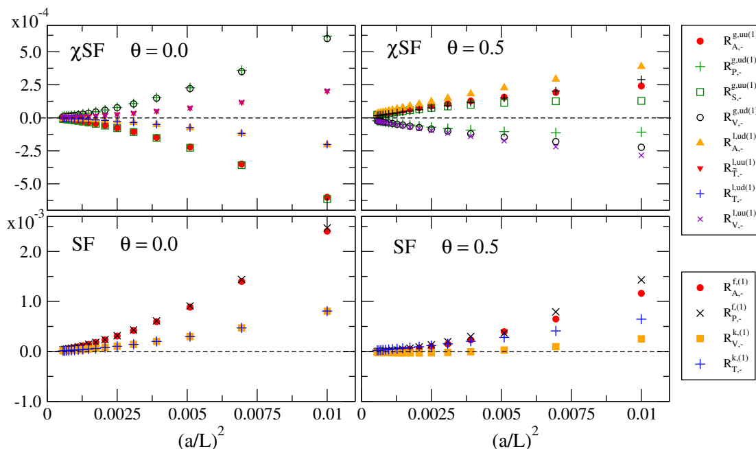
Figure 6. One-loop ratios (6.2) between correlation functions defined with reverted and correct projectors, respectively, for c_{sw} = 1 and both \theta = 0 and 0.5 . The factor C_F = 4/3 is included. The ratios for the \chi SF are displayed in the upper panels, while those for the SF are shown in the lower panels (note the scale difference).
