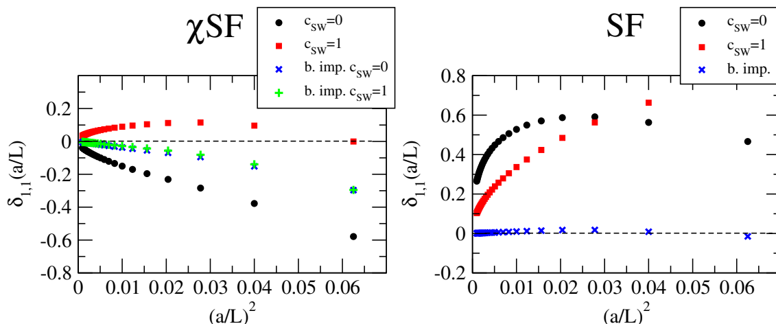
Figure 14. Cutoff effects \delta_{1,1} , eq. (8.12), for the \chi SF (left panel) and the standard SF (right panel). For both the SF and \chi SF we show the results with and without clover term. The legend “b. imp.” refers to c_t^{(1,1)} being set to the correct values, eqs. (5.29), otherwise it is set to zero.
