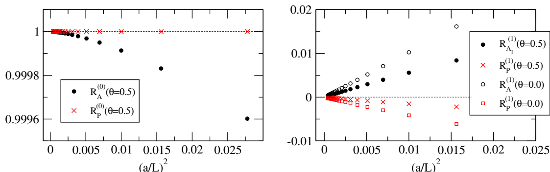
Figure 10. Ratios R_A and R_P at tree-level (left panel) and 1-loop (right panel) calculated for c_{sw}^{(0)} = 1 and C_F = 4/3 .
