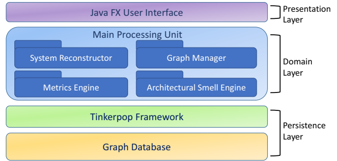
Fig. 2. Arcan Architecture
