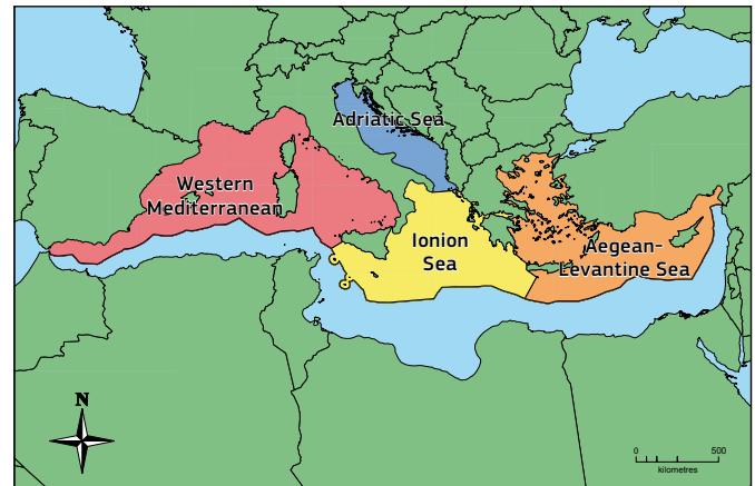
Figure 3.4.1 The Mediterranean Sea region with four sub-basins.
