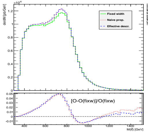
Figure 104: Mass distribution of \bar{t}t -system in the process us \rightarrow d c \bar{t}t around the resonance peak. The cuts listed in the left column of Table 60 have been applied.
