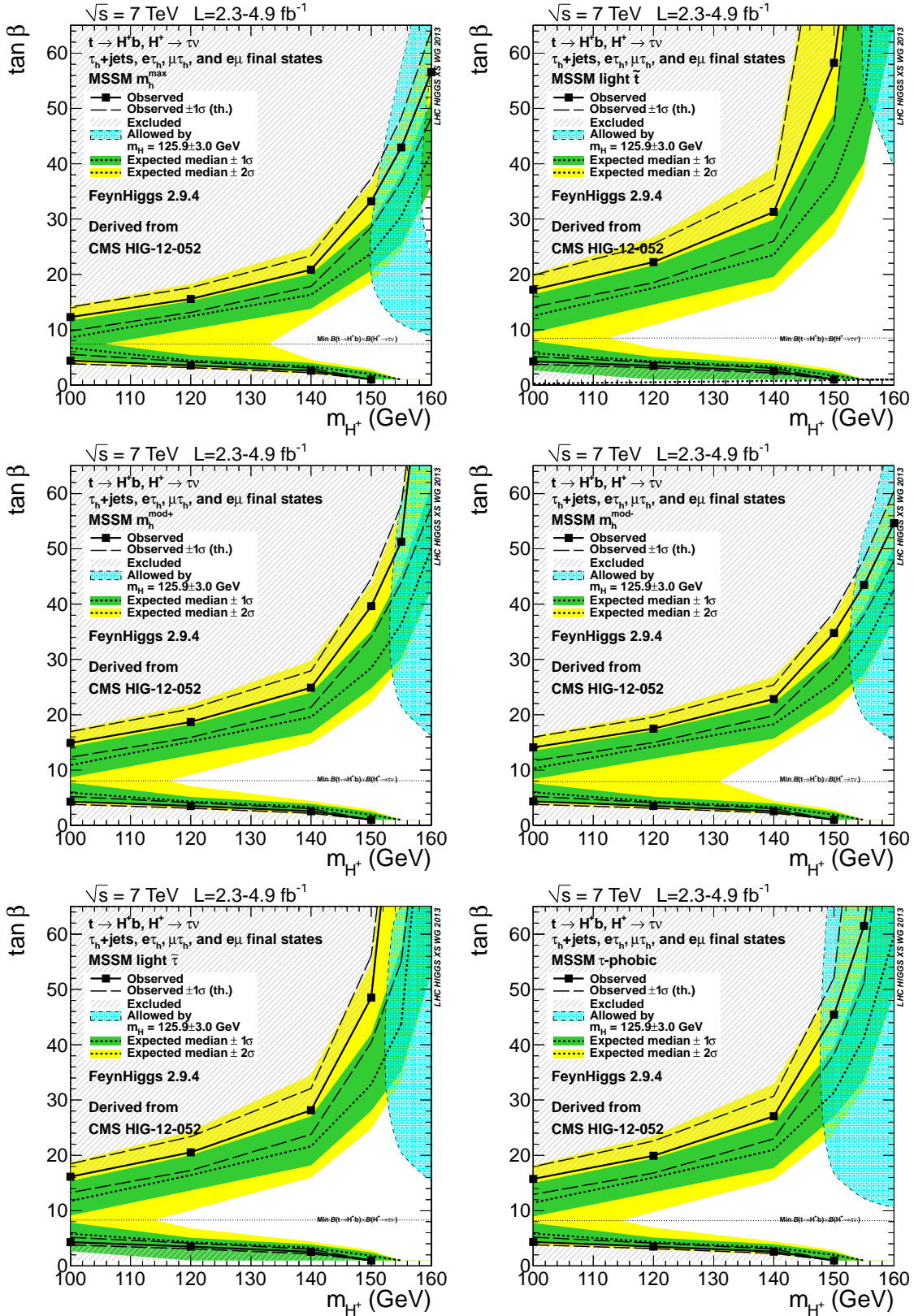
Figure 135: The exclusion limit derived from [719] for the light charged Higgs boson in the (M_{H^\pm}, \tan\beta) plane in the m_h^{\text{max}} scenario [16] (top left), in the light stop scenario [31] (top right), in the m_h^{\text{mod}+} scenario [31] (middle left) in the m_h^{\text{mod}-} scenario [31] (middle right) in the light stau scenario [31] (bottom left) and in the \tau -phobic scenario [31] (bottom right).
