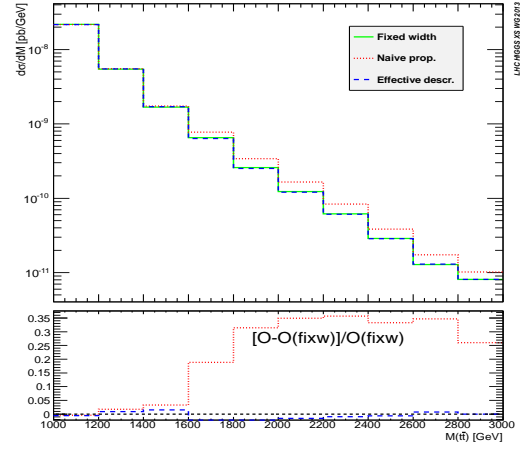
Figure 105: Mass distribution of \bar{t}t -system in the process us \rightarrow d c \bar{t}t at the high energy region. All cuts listed in Table 60 have been applied.
