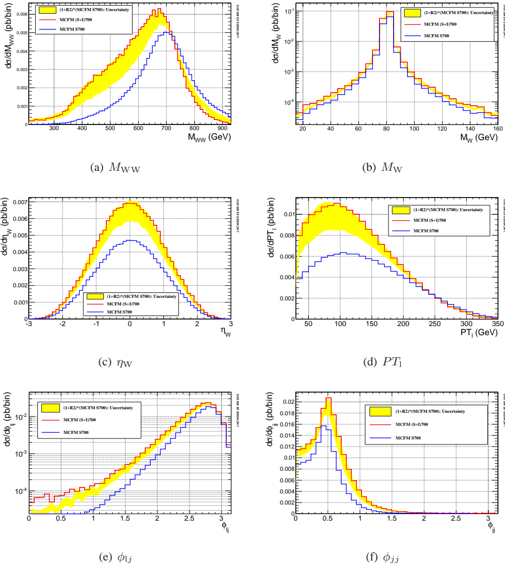
Figure 114: Reweighting MCFM gg \rightarrow H \rightarrow WW \rightarrow lv_1jj results to take into account interference effects at the generator level, for M_H = 700 GeV at the 8 TeV LHC, with p_T^1 > 30 GeV, p_T^j > 30 GeV, MET > 30 GeV, and |\eta_{l,j}| < 2.4 . Blue curves are for signal process, the red ones are for the signal plus continuum background, while the yellow bands correspond to the reweighted signal uncertainties Eqs.(301) and (302).
