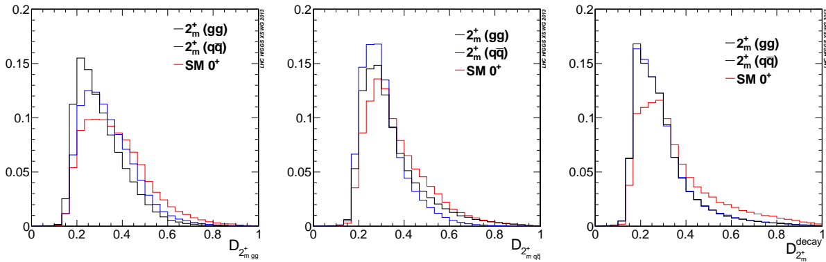
Figure 92: Distribution of the discriminants D_{2_m^{+}}^{gg} (left), D_{2_m^{+}}^{q\bar{q}} (middle), D_{2_m^{+}}^{\text{decay}} (right) evaluated with three different samples: SM Higgs boson, spin-two produced through gluon-gluon fusion and produced through q\bar{q} annihilation.
