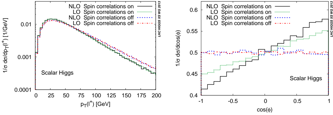
Fig. 45: Next-to-leading-order cross sections differential in p_T(l^+) (left panel) and in and \cos \phi (right panel) for t\bar{t}H events with or without spin correlation effects. For comparison, also the leading-order results without spin-correlation effects are shown. Events were generated with AMC@NLO, then decayed with MADSPIN, and finally passed to HERWIG for parton showering and hadronization.
