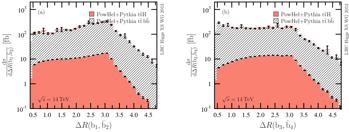
Fig. 53: \Delta R distance in the pseudorapidity–azimuthal angle plane between the two hardest b-jet pairs, and between the two second-hardest b-jet pairs with one b- and one \bar{b} -tagged jet in the pairs. The t\bar{t}H and the t\bar{t}b\bar{b} distributions after POWHEL+PYTHIA are shown by pink and shaded black histograms, respectively. When comparing the two panels a difference in the shape of the distributions is clearly visible. The error bars represent the statistical uncertainty of the events.
