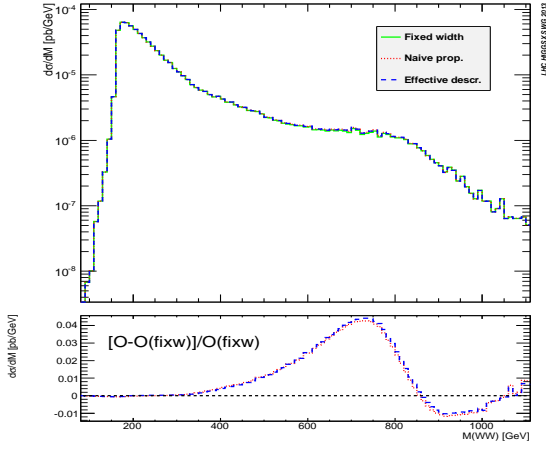
Figure 106: Mass distribution of the reconstructed WW -system in the process gg \rightarrow W^+W^- \rightarrow e^+\nu_e\mu^+\nu_\mu , around the resonance peak. The cuts listed in Table 61 have been applied.
