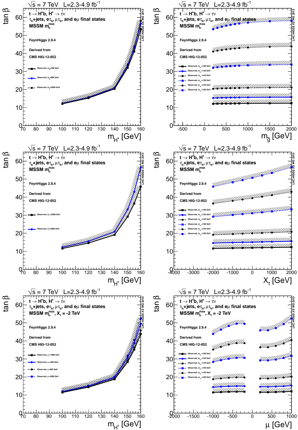
Figure 138: The effect of varying M_g on the experimentally excluded region in the m_h^{\text{max}} scenario (top left and right), the effect of varying X_t (middle plots), and the effect of varying the \mu parameter with X_t = -2 \text{ TeV} (bottom plots).
