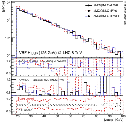
Fig. 36: Veto-jet transverse momentum (left) and rapidity (right) distributions. Main frame and upper inset: AMC@NLO results; middle inset: ratio of POWHEG results over AMC@NLO+HERWIG6; lower inset: AMC@NLO+HERWIG6 scale and PDF variations.
