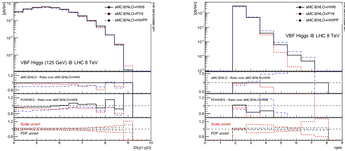
Fig. 34: Rapidity separation of the two tagging jets (left) and exclusive jet-multiplicity (right). Main frame and upper inset: AMC@NLO results; middle inset: ratio of POWHEG results over AMC@NLO+HERWIG6; lower inset: AMC@NLO+HERWIG6 scale and PDF variations.
