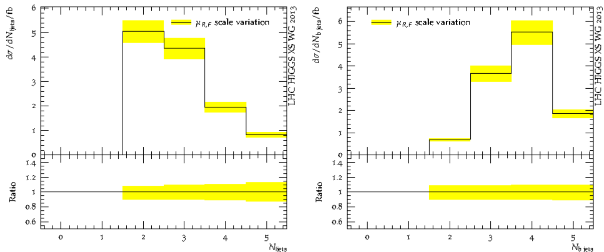
Fig. 41: The number of light (left panel) and b jets (right panel) in the acceptance region for t\bar{t}H events at the 8 TeV LHC. Uncertainties due to renormalization and factorization scale variations (yellow band) as given in an MC@NLO simulation are also indicated.
