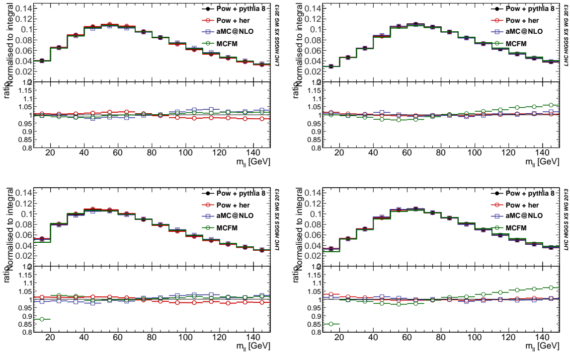
Fig. 27: Parton showering/modelling uncertainties in the m_{ll} distribution in (top left) SR1/2 in DF 0j analysis, (top right) SR1/2 in DF 1j analysis, (bottom left) SR in SF 0j analysis, and (bottom right) SR in SF 1j analysis. POWHEG + PYTHIA8/HERWIG is shown along with MCFM. All ratios are with respect to POWHEG + PYTHIA8.
