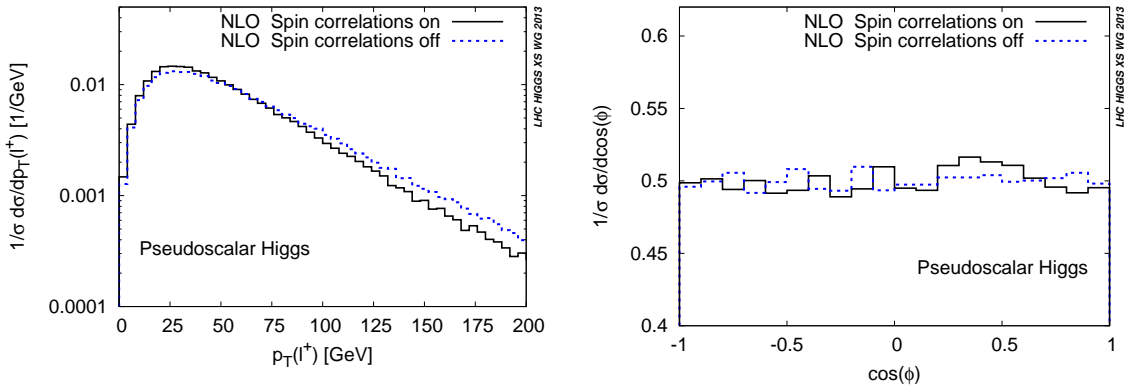
Fig. 46: Next-to-leading-order cross sections differential in p_T(l^+) (left panel) and in and \cos(\phi) (right panel) for t\bar{t}A events with or without spin-correlation effects. Events were generated with AMC@NLO, then decayed with MADSPIN, and finally passed to HERWIG for parton showering and hadronization.
