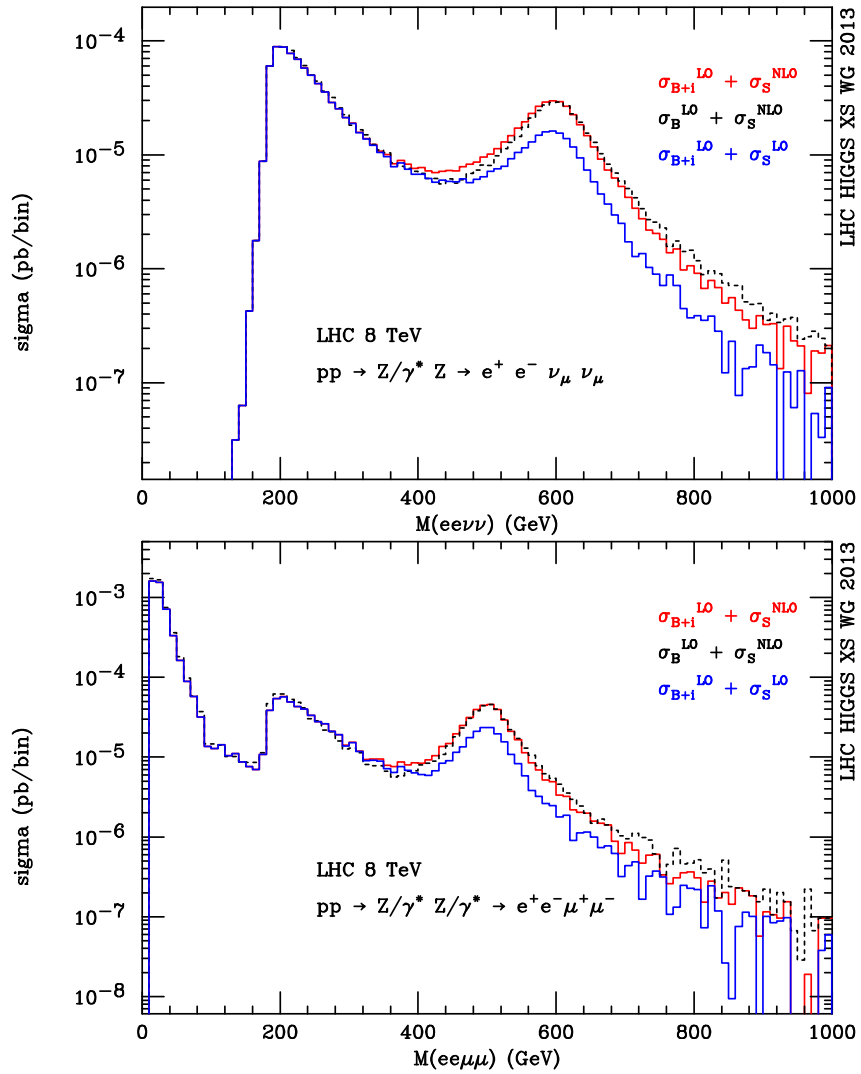
Figure 113: Invariant mass distributions for pp \rightarrow 4l in different channels as obtained from MC@NLO for the signal S and MADLOOP for the background and interference B + i . Basic acceptance cuts applied.
