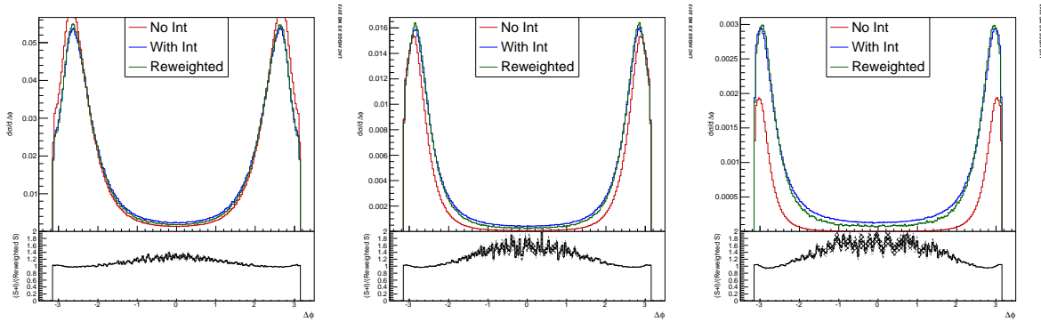
Figure 118: Distributions of the dilepton azimuthal opening angle \Delta\phi_{\ell\ell} showing the effect of the interference and the result of the reweighting procedure after cuts, corresponding to a Higgs mass of M_H = 400 GeV (left), 600 GeV (middle), 900 GeV (right).
