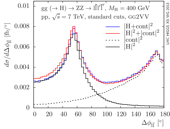
Figure 109: Azimuthal opening angle \Delta\phi_{\ell\ell} distributions for gg (\rightarrow H) \rightarrow ZZ \rightarrow \ell\bar{\ell}'\ell' in pp collisions at 7 TeV for M_H = 400 GeV. Other details as in Figure 108.
