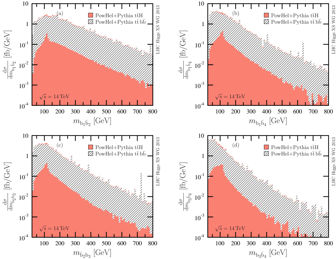
Fig. 52: Invariant mass of the four possible b -jet pairs with one b - and one \bar{b} -tagged jet in the pairs. The t\bar{t}H and the t\bar{t}b\bar{b} distributions after POWHEL+PYTHIA are shown by pink and shaded black histograms, respectively. Peaks around the Higgs mass are visible in the t\bar{t}H distributions.
