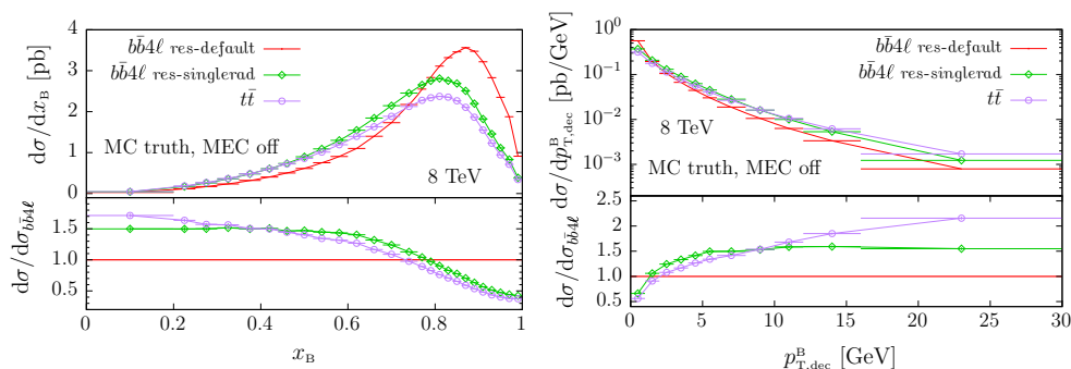
Fig. 22 Predictions for the B fragmentation function and transverse-momentum distribution of the B hadron in the top decay frame, p_{T,dec}^B obtained with the bb41 generator in its default mode employing the multiple-radiation scheme (res-default), without employing this scheme (res-singlerad) and corresponding predictions obtained
