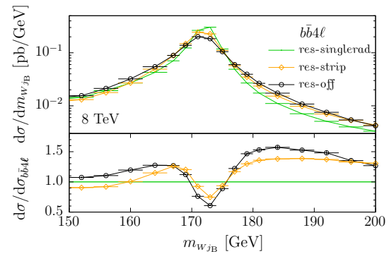
Fig. 4 Invariant mass of the Wj_B system obtained with the bb4l generator. We compare our resonance-aware predictions without employing the multiple-radiation scheme ( res-singlerad ) against the “traditional”, i.e. resonance-unaware, implementation ( res-off ) and a prediction where any resonance information is stripped off the Les Houches event file ( res-strip ). In the ratio plot we illustrate relative deviations with respect to res-singlerad
