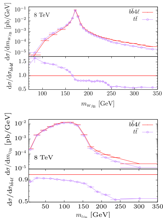
Fig. 10 Invariant mass of the W_{j_B} (top) and of the l_{j_B} (bottom) systems. Comparison of NLO+PS predictions obtained with the bb4l ( bb4l ) and the hvq ( tt ) generators. In the ratio plot we illustrate relative deviations with respect to the bb4l prediction
