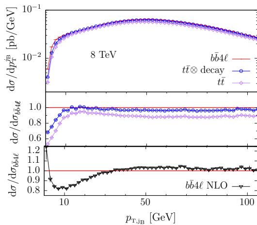
Fig. 14 Distribution in the b -jet transverse momentum: comparison of NLO+PS predictions obtained with the three generators bb4l ( bb4l ), tt \otimes decay ( tt \otimes decay) and tt ( tt ). The middle frame illustrates relative NLO+PS deviations with respect to the bb4l prediction, while the lower frame compares bb4l versus corresponding fixed-order NLO results
