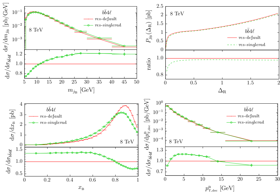
Fig. 21 Mass (left top) and profile (right top) of the b -jet, j_B , and for the B fragmentation function (left bottom) and transverse-momentum distribution of the B hadron in the top decay frame, p_{T,dec}^B (right bottom). Absolute predictions and ratios as in Fig. 20
