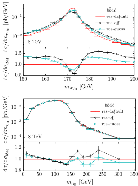
Fig. 3 NLO+PS predictions for the invariant mass of the Wj_B (top) and of the lj_B (bottom) systems obtained with the new bb4l generator. We compare our default resonance-aware predictions ( res-default ) against the “traditional”, i.e. resonance-unaware, implementation ( res-off ) and a prediction where the event-by-event resonance information is obtained from a guess based on kinematics. In the ratio plot we illustrate relative deviations with respect to res-default
