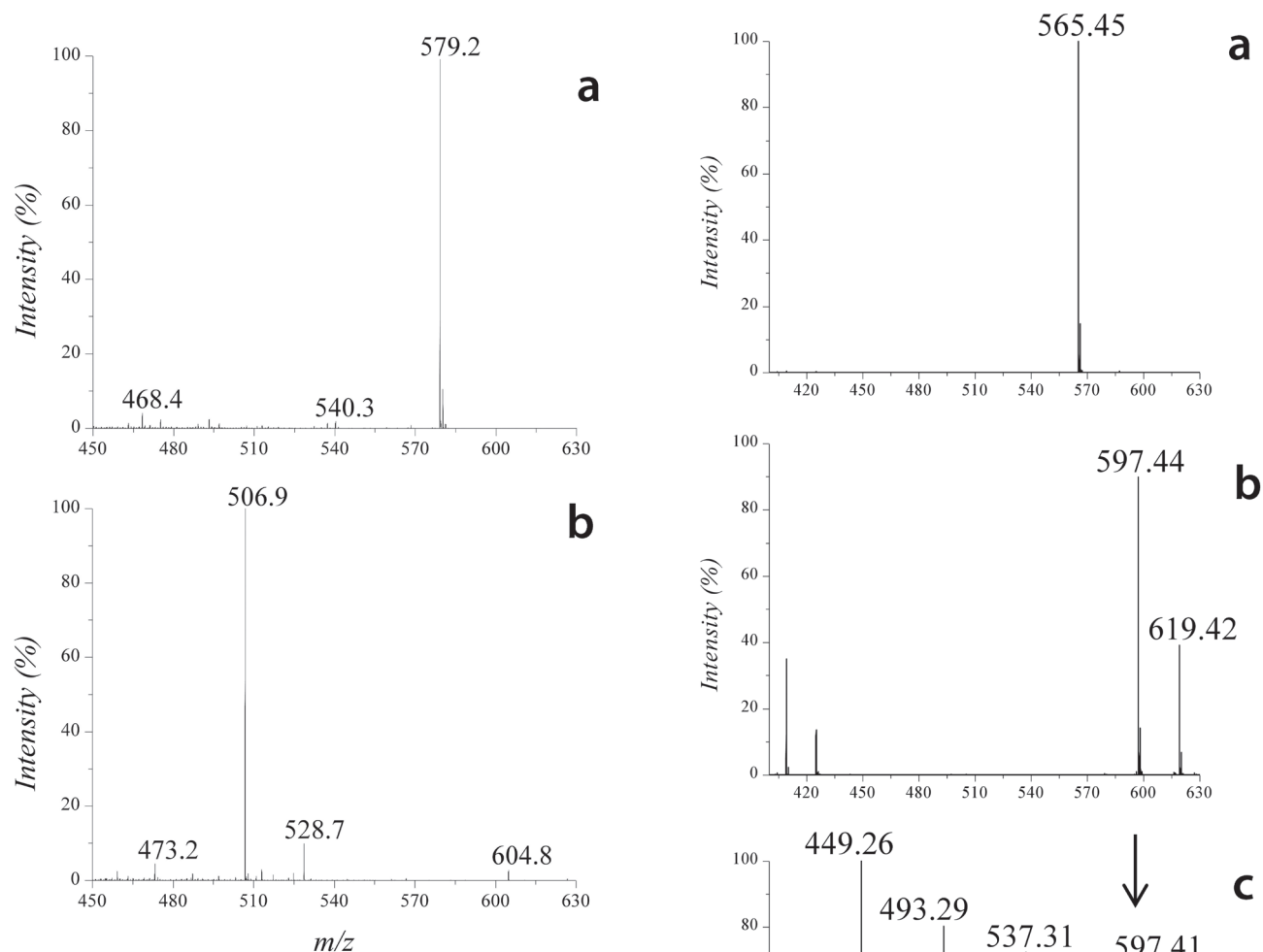
Figure 8. ESI-MS spectra of HPLC elution peaks 1 (a) and 2 (b) of the sample Torre del Greco. The most intense peaks are labelled by their mass-charge ratio ( m/z ).
