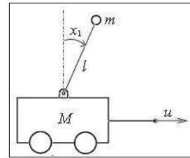
Figure 2: Inverted pendulum on a cart.
