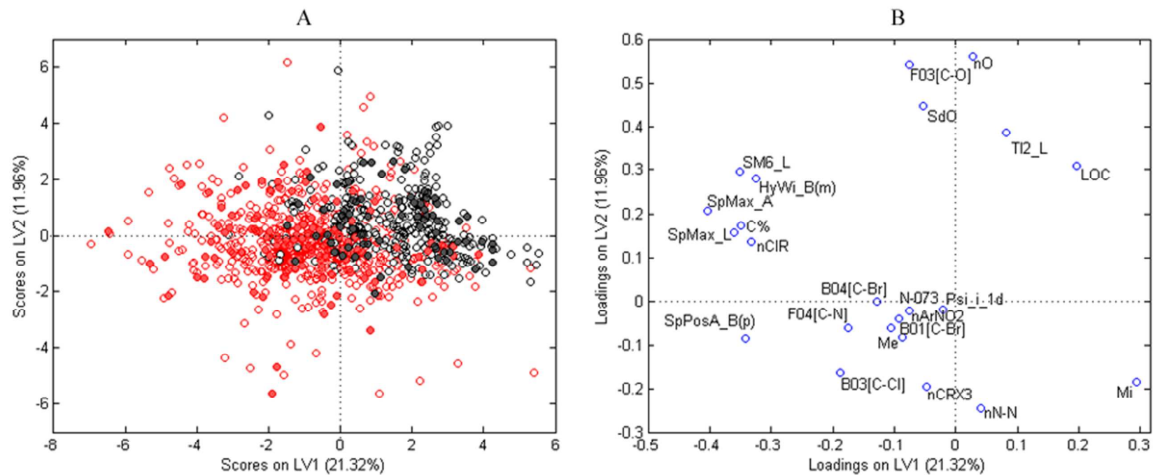
Figure 2. Scores plot (A) and Loadings plot (B) of the first and second Latent Variables of the PLSDA model (Explained Variance equal to 33%). Ready biodegradable molecules are coloured in black, not ready biodegradable in red; training molecules are marked with empty circles, test molecules with full circles. Labels of the molecular descriptors refer to symbols listed in Table 7.
