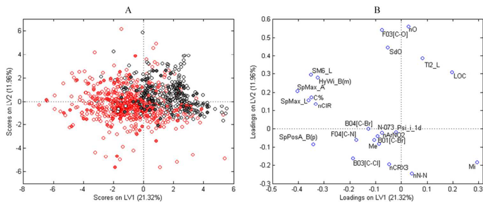
Figure 2: Scores plot (A) and Loadings plot (B) of the first and second Latent Variables of the PLSDA model (Explained Variance equal to 33%). Ready biodegradable molecules are coloured in black, not ready biodegradable in red; training molecules are marked with empty circles, test molecules with full circles. Labels of the molecular descriptors refer to symbols listed in Table 7.
