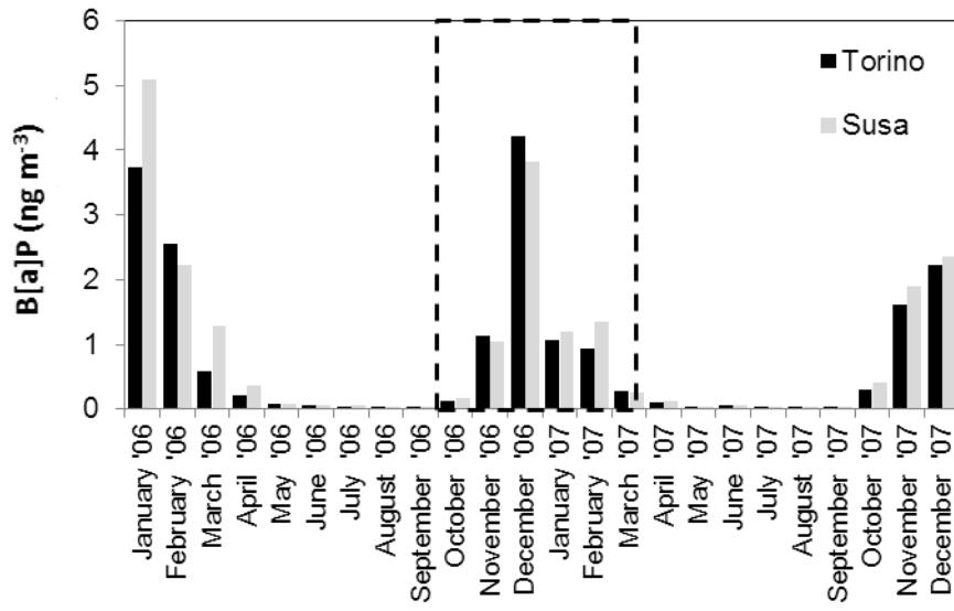
Figure 3: Monthly trends for concentrations of B[a]P.
