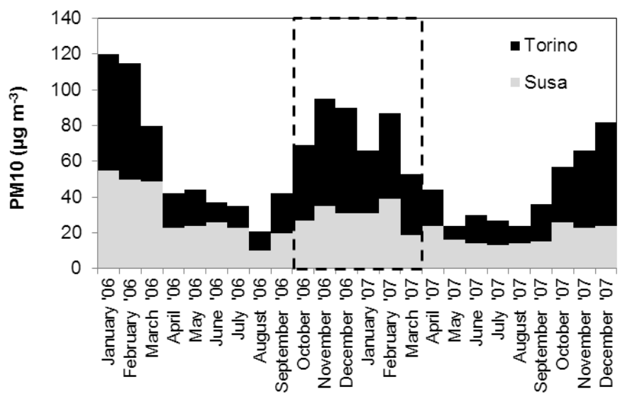
Figure 2: Monthly trends for concentrations of PM10.
