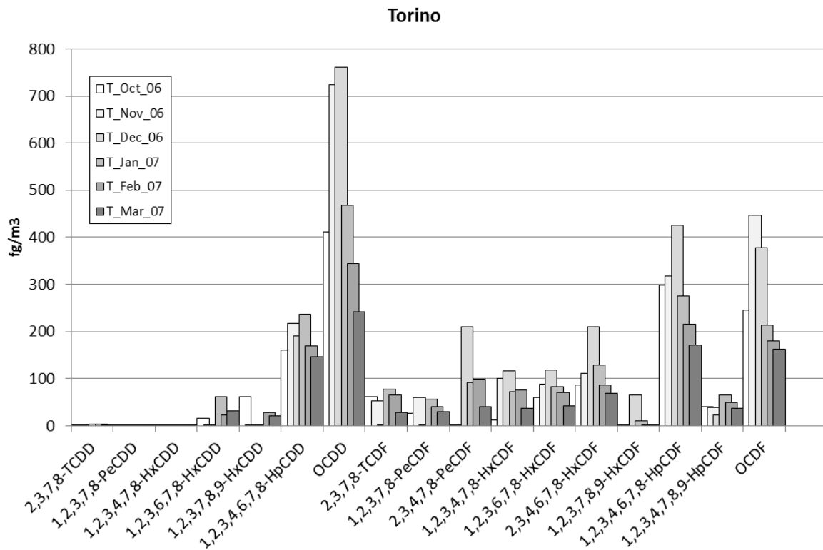
Figure 5: Monthly concentrations of the 2,3,7,8-chlorinated PCDD/Fs in Susa (S) and Torino (T).
