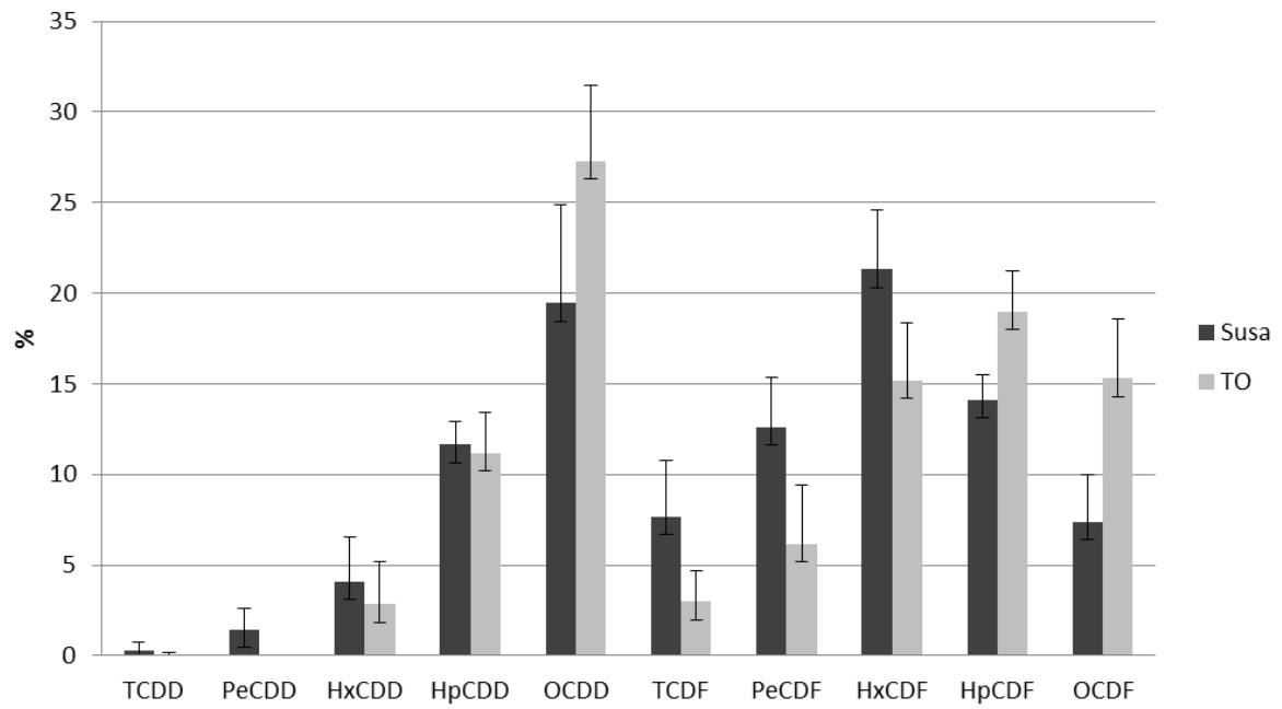
3 Figure S5: Mean 2,3,7,8-fingerprints determined for Torino and Susa.
