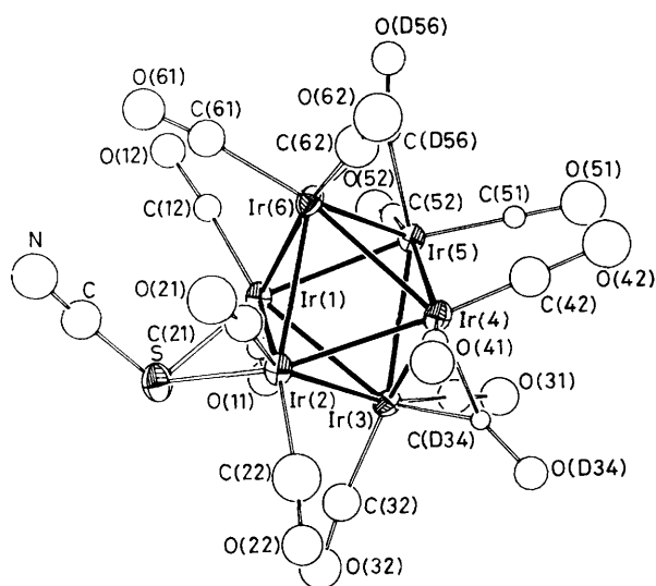
Figure 3. ORTEP drawing of [Ir 6 (CO) 14 (μ-SCN)] - (4); thermal ellipsoids are drawn at 30% probability
