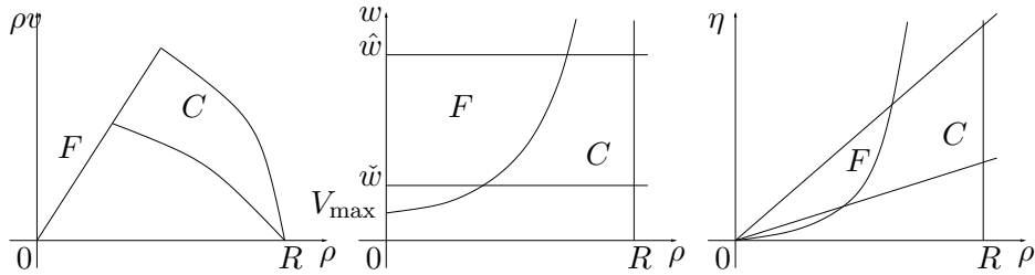
Figure 2: The phases F and C in the coordinates, from left to right, (\rho, \rho v) , (\rho, w) and (\rho, \eta) .
