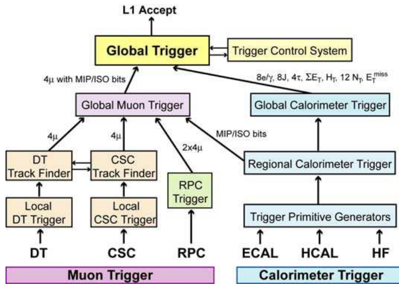
Figure 1.16.: Architecture of Level-1 Trigger [3]
