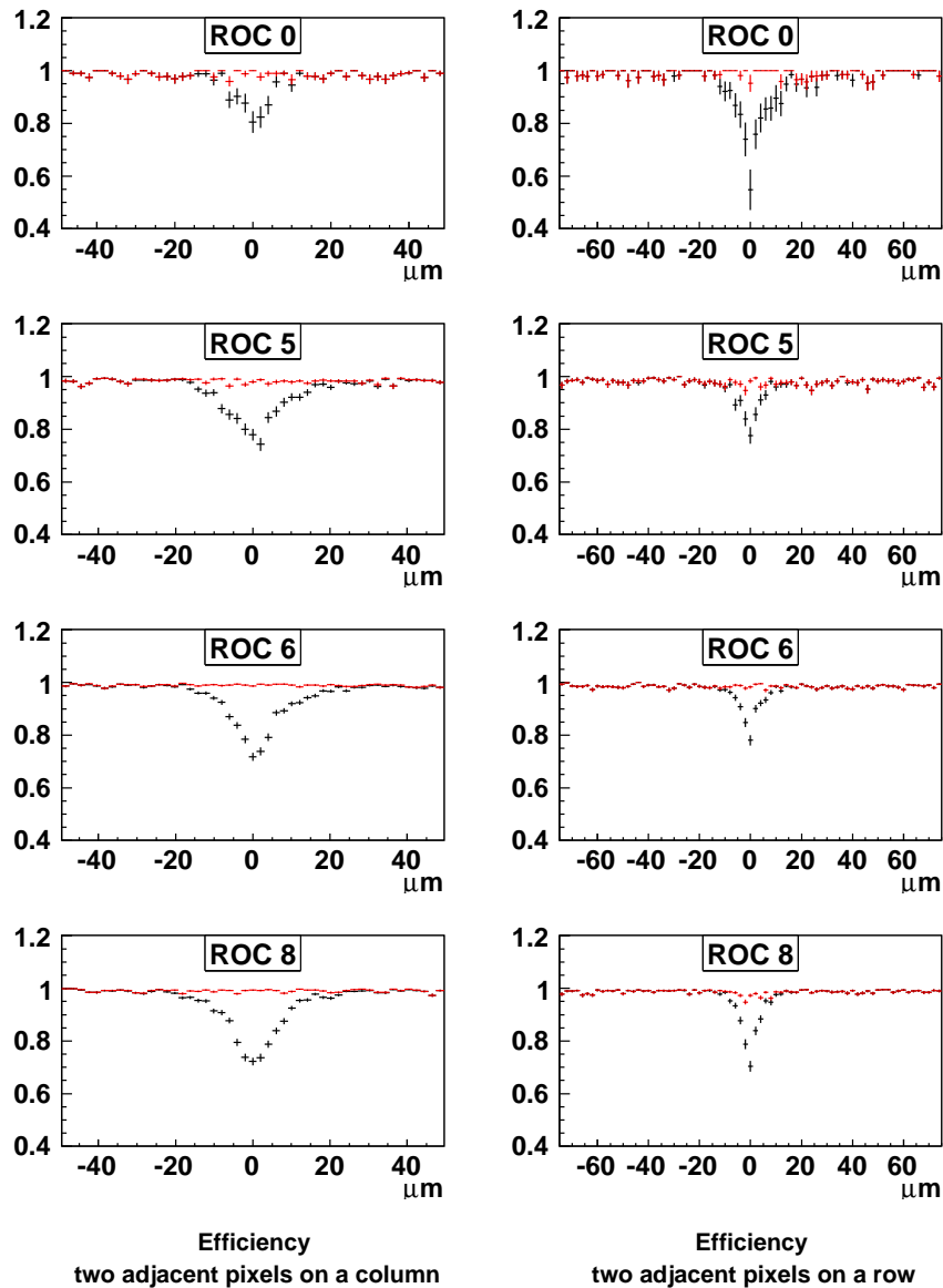
Figure 2.9.: Detection efficiency as a function of the distance track impact point from the boundary of the two adjacent pixel on the same column (histograms on the left), or on the same row (histograms on the right)
