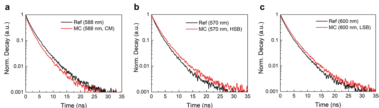
Figure 3. Time-resolved PL intensity of PSiO 2 MC and reference structures coated with PAH-RhoB via electrostatic nanoassembly. a, c) Time-resolved PL of a) tuned cavity mode peaked at 588 nm, b) detuned high-energy side stopband mode peaked at 570 nm, and c) detuned low-energy side stopband mode peaked at 600 nm.
