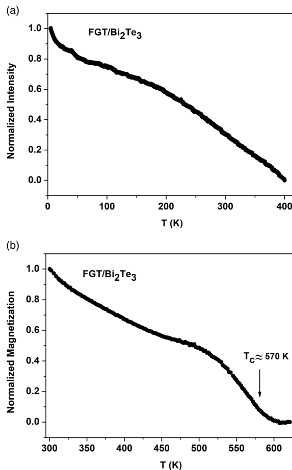
Fig. 7 Temperature dependence of the Normalized magnetization for 17 nm thick FGT/ \text{Bi}_2\text{Te}_3 (a) in the temperature range 5 K–400 K with normalization M - M_{400 \text{ K}} / (M_{5 \text{ K}} - M_{400 \text{ K}}) and (b) in the temperature range 300 K–620 K with normalization M - M_{620 \text{ K}} / (M_{300 \text{ K}} - M_{620 \text{ K}}) .
