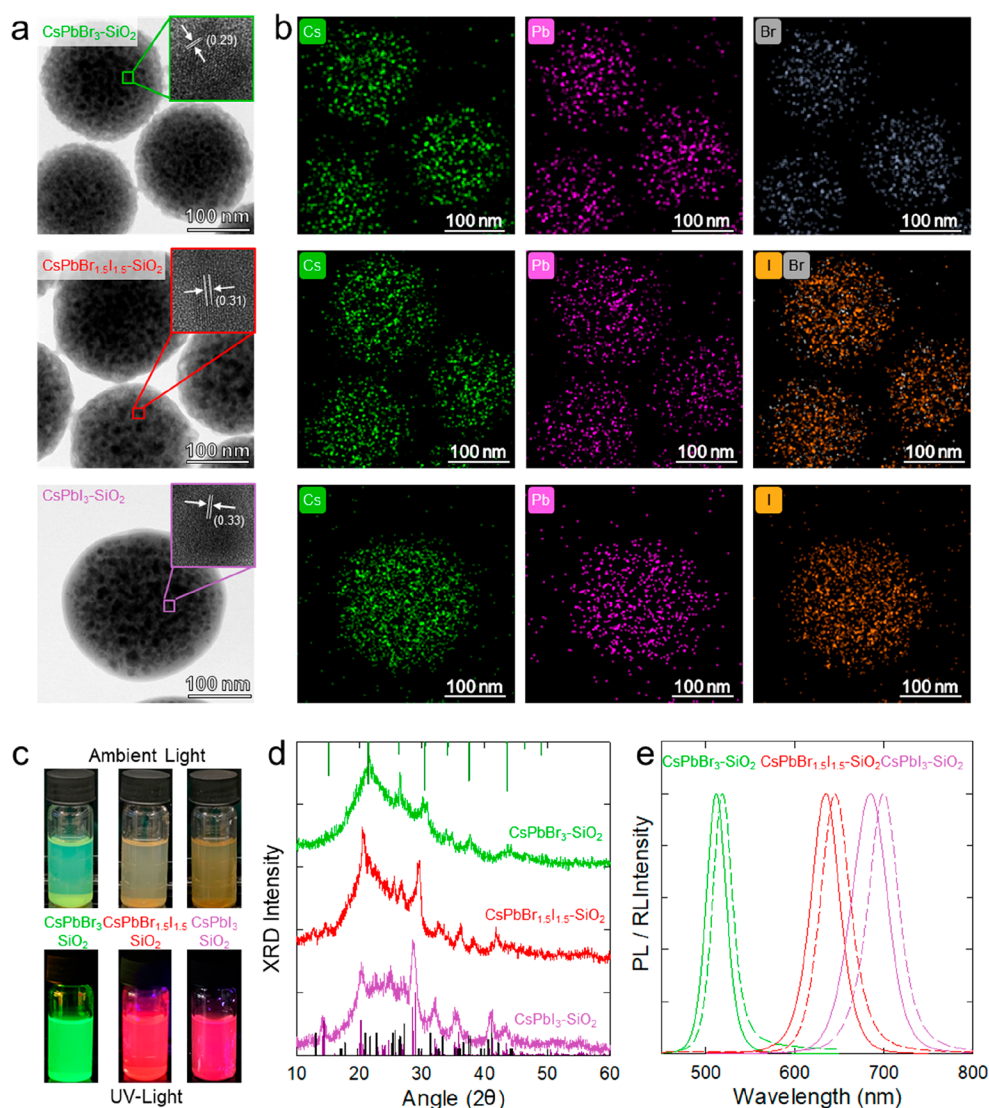
Figure 1. (a) TEM images of CsPbBr 3 -SiO 2 , CsPbBr 1.5 I 1.5 -SiO 2 , and CsPbI 3 -SiO 2 NSs. (b) HAADF-STEM images and elemental mappings on the same samples highlighting the presence of Cs (green), Pb (purple), Br (gray), and I (yellow) inside the NSs. (c) Photographs of CsPbBr 3 -SiO 2 , CsPbBr 1.5 I 1.5 -SiO 2 , and CsPbI 3 -SiO 2 in aqueous solution taken under ambient illumination (top pictures) and under UV illumination (bottom pictures). (d) XRD patterns of CsPbBr 3 -SiO 2 (green line), CsPbBr 1.5 I 1.5 -SiO 2 (red line), and CsPbI 3 -SiO 2 (purple line). The diffraction patterns of cubic CsPbBr 3 (ICSD 97852, green), orthorhombic \gamma -phase (ICSD 434338, violet line), and orthorhombic \delta -phase (ICSD 250744, black line) of CsPbI 3 are also reported as references. (e) Normalized PL (solid lines) and RL (dashed lines) spectra of the same samples in dry powder form (excitation wavelength, 405 nm for PL; X-ray irradiation at 20 kV for RL).
