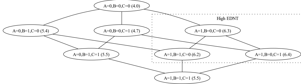
■ Figure 3 Visualization of Example 3: The state space graph (same graph as in Figure 1b, but presented slightly differently) is annotated with EDNTs for each node (in parentheses) and a subset of nodes with relatively high EDNT values is highlighted. Sentry states are high EDNT states to which transitions from low EDNT states are possible and such a transition increases the risk of an imminent cascade. Some states with high EDNT tend to occur in the middle of a cascade which motivates using the REDNT metric. In this example, transitioning from (A = 0, B = 0, C = 0) to (A = 1, B = 0, C = 0) may trigger an alarm in B which in turn may trigger an alarm in C , resulting in a cascade (note that only transitions along the edges in the state space graph are possible).
