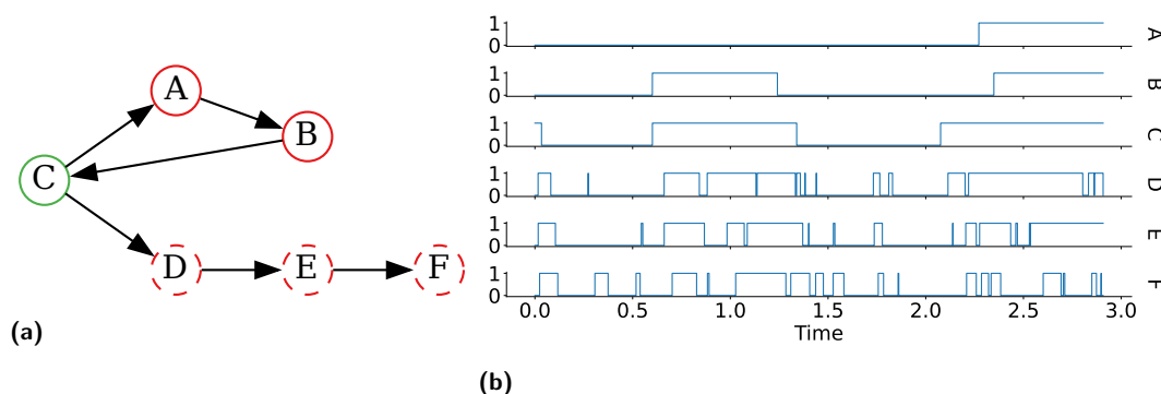
■ Figure 5 (a) Graph \mathcal{G} of a CTBN model consisting of six processes. The graph G contains the cycle (A, B, C) as well as the chain (D, E, F) . See the caption of Figure 4 for an explanation of the node colors.
