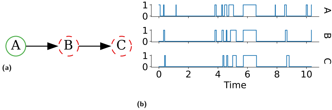
■ Figure 4 (a) depicts the graph \mathcal{G} of a CTBN. Its CIMs are in Table A1 in the appendix. Slow processes are represented by solid line nodes, while fast processes are represented by dashed line nodes. Colors describe the most likely sentry state, s = (s_1, s_2, s_3) , in this system: If a node is green, the corresponding alarm is 1 ( on ) in s . If a node is red, the corresponding alarm is 0 ( off ) in s . (b) shows an example trajectory from the CTBN represented in Figure 4a. Each function in the plot represents the evolution of one of the three binary processes, A , B , and C .
