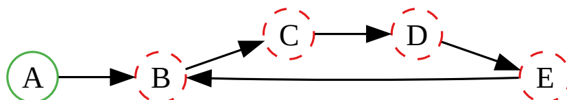
■ Figure A2 Graph \mathcal{G} of a CTBN model consisting of five processes, including a cycle.
