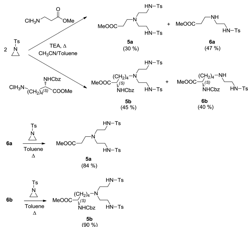
Scheme 1 Synthesis of amino acid derived 4 substituted 1,4,7-triazheptanes 5a and 5b .
