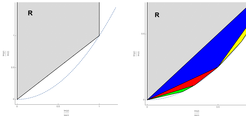
Figure 1. The plot to the left shows the chamber R (shaded grey region) for 1/\Phi_{10} , i.e. t = 1 . The dashed line corresponds to the boundary of the Siegel upper half plane; the solid lines correspond to (4.15). The plot to the right shows the tessellation of \mathbb{H}_2 , which is produced by considering further lines in H_1(1) ; each colored region represents a new chamber which is surrounded by the appropriate divisor in (4.14).
