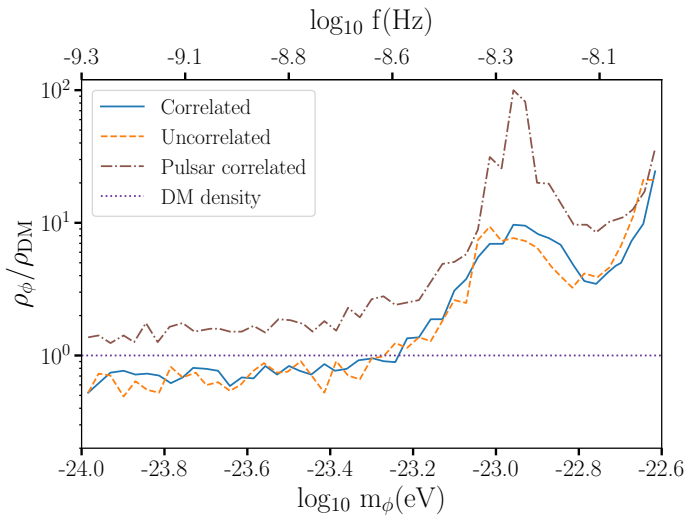
Fig. 23: Constraints on the ULDM density \rho_\phi normalised to the DM background value \rho_{\text{DM}} = 0.4 \text{ GeV/cm}^3 . The blue, orange and brown lines represent the 95% Bayesian upper limit on \rho_\phi , obtained from the EPTA DR2new dataset with the correlated, uncorrelated and pulsar correlated analysis, respectively. The purple dotted line shows the fiducial local DM density value.
