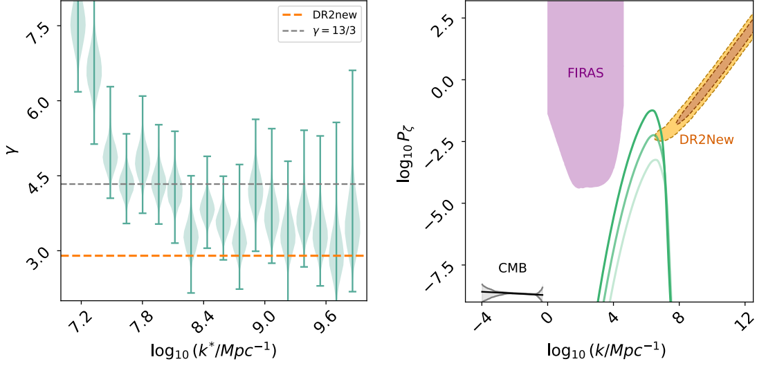
Fig. 19: Results for the monochromatic curvature perturbations described by Eq. 24. Left panel: recovered slopes \gamma of a simple power-law model as a function of characteristic scale k^* of the injected GWB generated by the monochromatic curvature perturbations. The horizontal lines show the theoretical value of \gamma from a population of circular, GW-driven SMBHBs (grey) and the one obtained in PaperIII (orange). Right panel: 1\sigma and 2\sigma contours of the posterior distributions on the amplitude A_\zeta and characteristic scale of fluctuations k^* for DR2new (orange colour). The posterior distribution is overlaid with the current constraints on the primordial power spectrum using Planck data (CMB). The grey colour depicts the 2\sigma -confidence intervals. The purple shaded area represents the bounds from spectral distortions (Chluba et al. 2012). For comparison in green we place the prediction of the primordial spectrum of scalar perturbations in the two-field model of inflation described in Braglia et al. (2020) for a range of the model parameters. All three models result in PBH mass functions peaked at \sim 35 M_\odot with the brightest line corresponding to the dark matter fraction of PBHs of \sim 0.01 .
