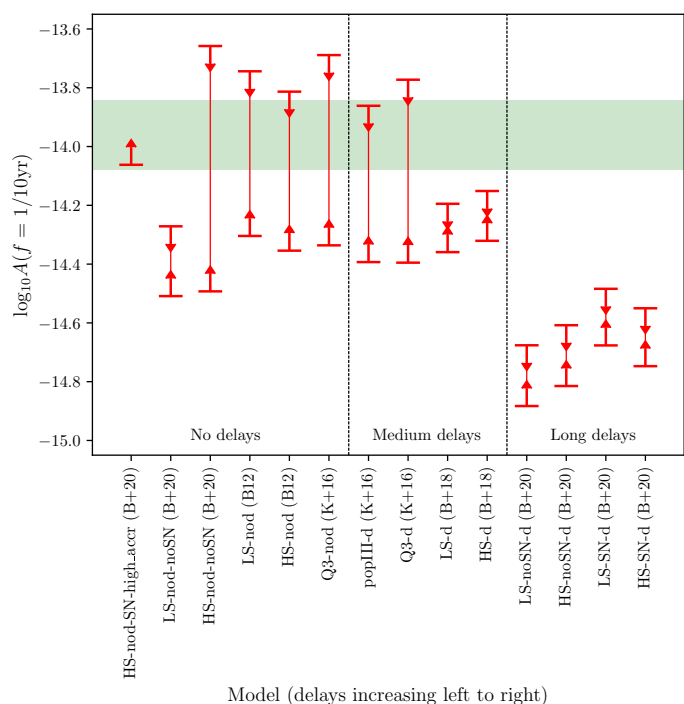
Fig. 9: Predictions for the GWB characteristic strain amplitude at f = 1/10\text{yr} from a range of SAMs published in the literature, assuming quasicircular orbits and no environmental interactions (i.e. \gamma = 13/3 ), but different physical prescriptions for the delays (increasing from left to right) between galaxy mergers and black hole mergers. The “no delays”, “medium delays” and “long delays” models correspond respectively to the classes of models (i), (ii) and (iii) defined in the text. The ranges account for the finite resolution of the models. The shaded area is the DR2new 95% confidence bound. More details about the models are provided in the text.
